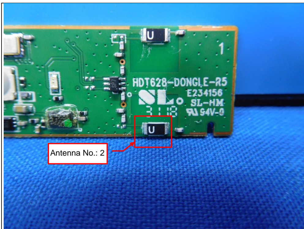
Antenna No. 2
