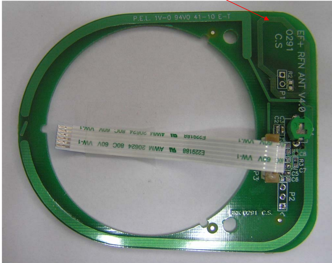
Photograph No.7 Antenna's PCB with NID antenna
