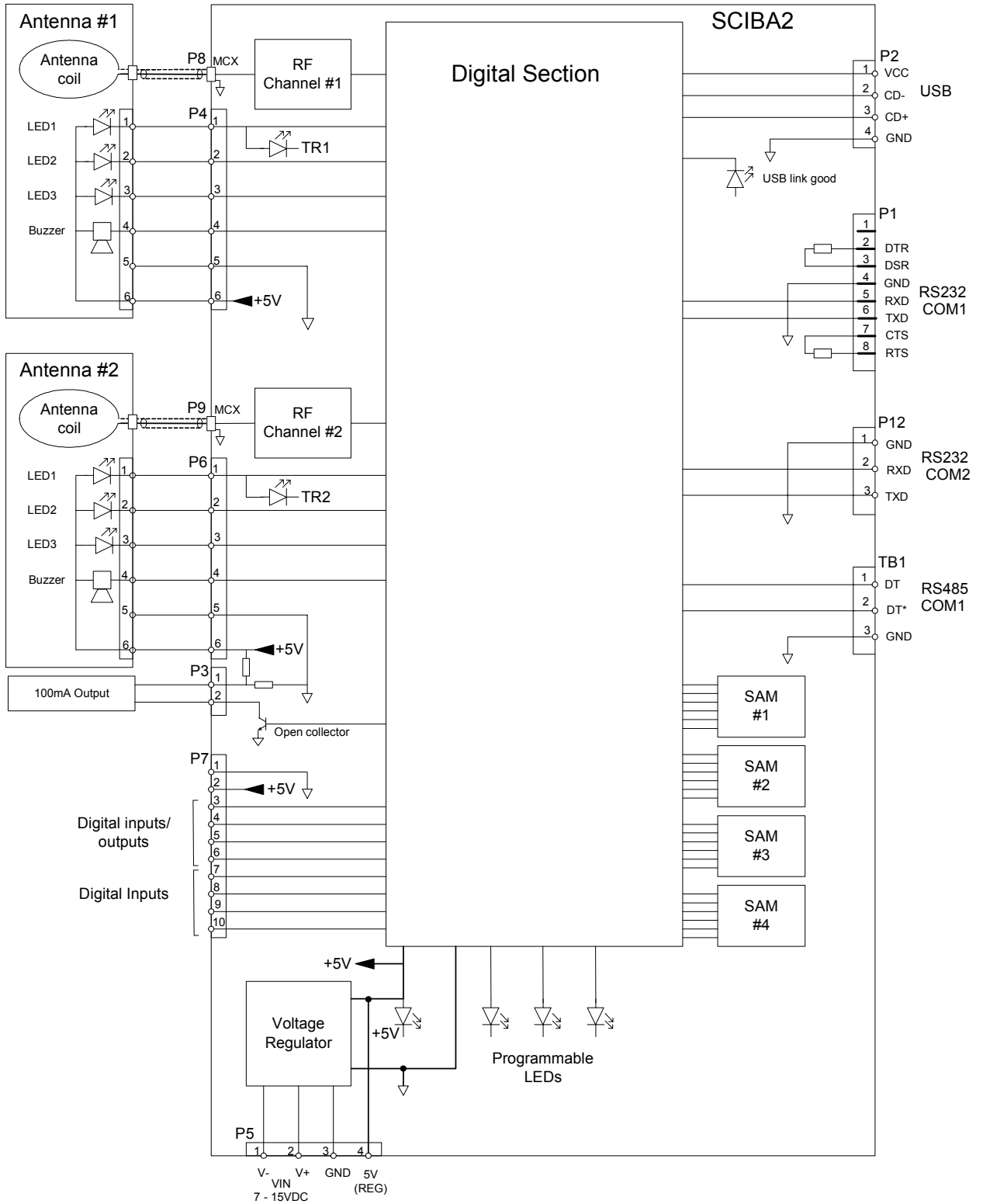
SCIBA2 – Reader Block Diagram
