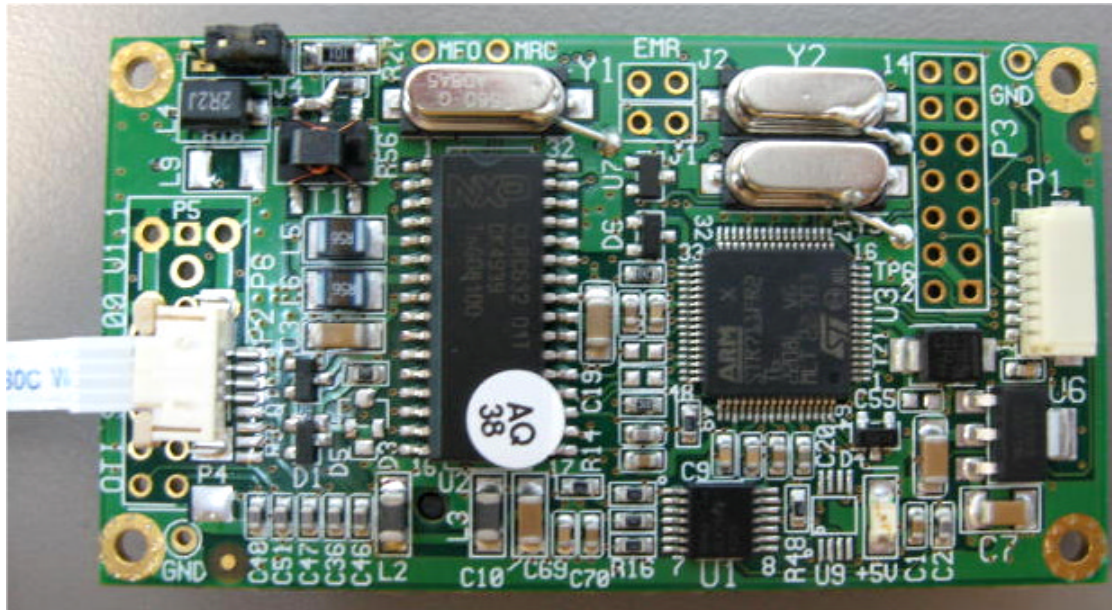
Photograph No.2 SCI6100M card reader PCB top view
