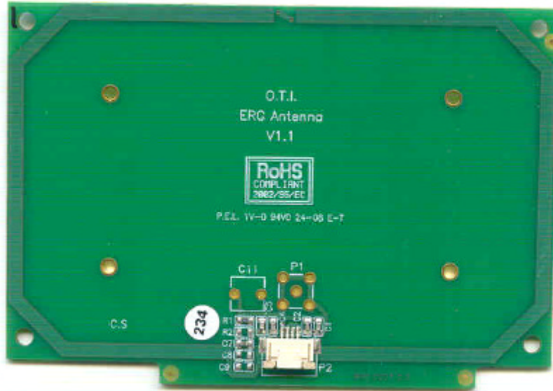
Photograph No.5 SCI6100M antenna without metal cover and ferrite
