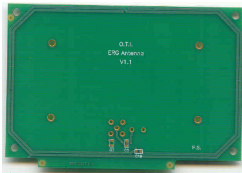
Photograph No.6 SCI 6100M antenna second side
