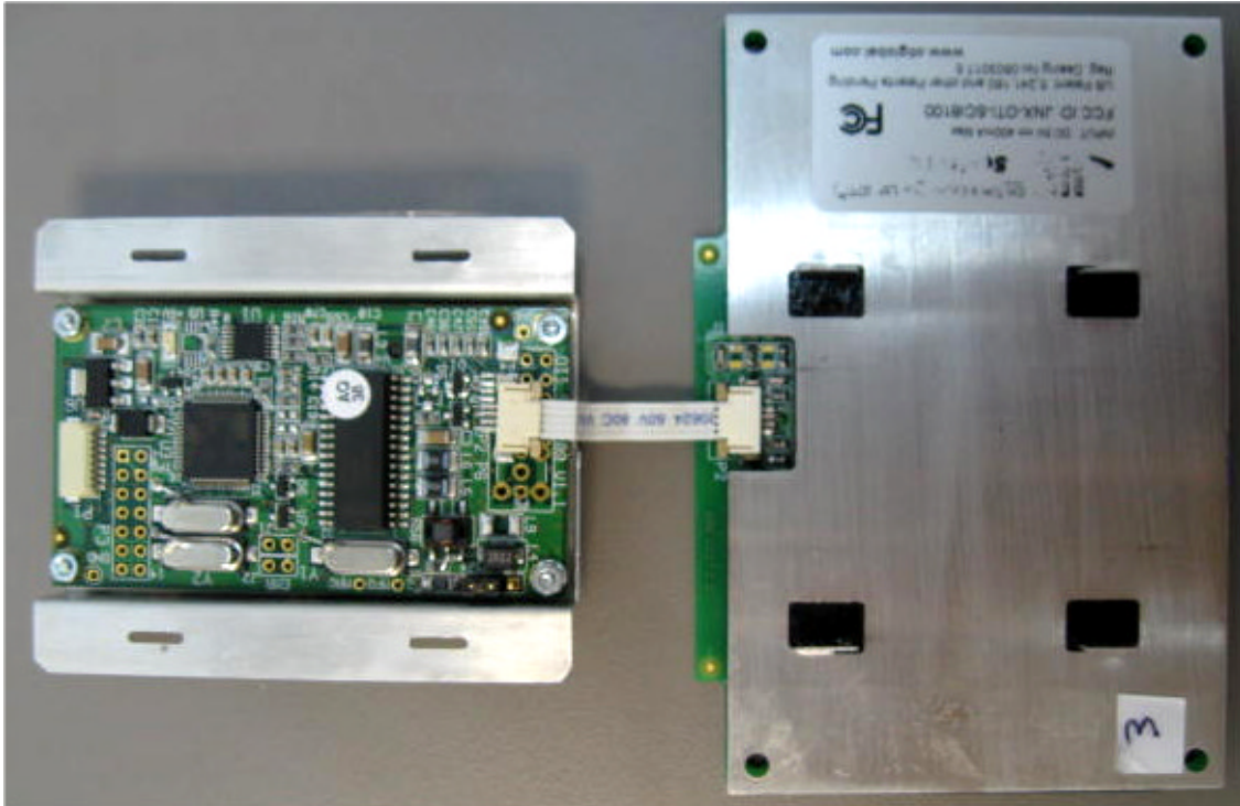
Photograph No.1 Card reader SCI6100M internal view
