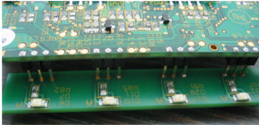
Photograph No.5 Daughter PCB close view
