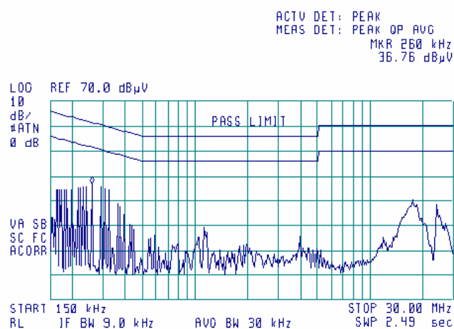
Plot 7.3.2 Conducted emission measurements at the EUT power lines
