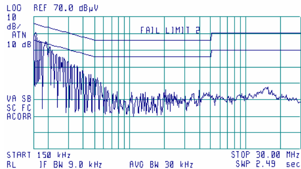
Plot 8.1.4 Conducted emission measurements at the laptop power lines
