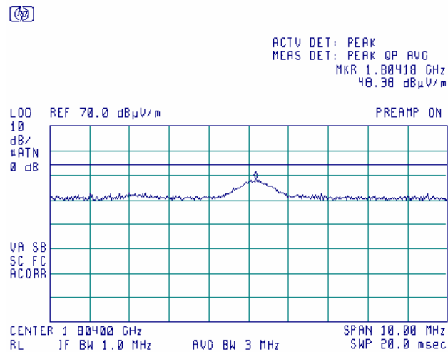
Plot 7.1.9 Radiated emission measurements at the third harmonic frequency
