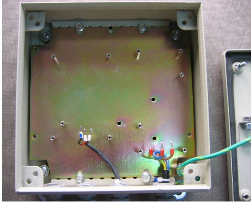
Photograph No.7 Site controller case internal view without PCBs
