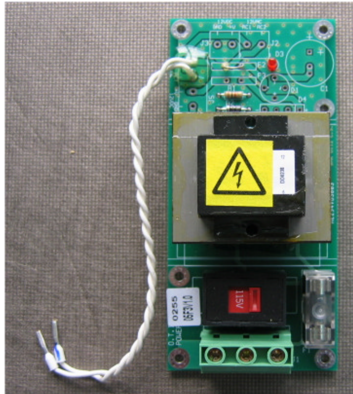
Photograph No.5 Second PCB front view
