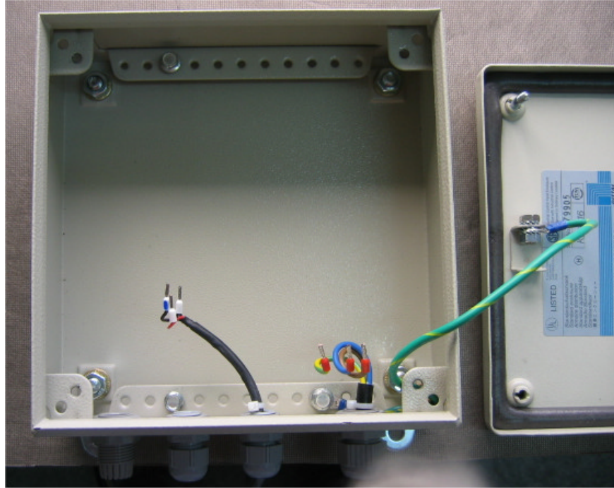
Photograph No.8 Site controller case internal view
