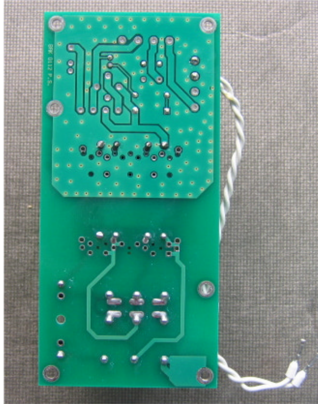
Photograph No.6 Second PCB bottom view
