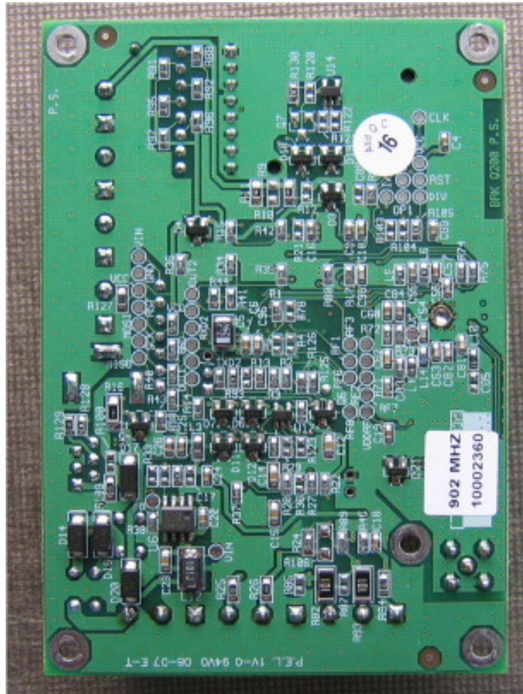
Photograph No4 Site controller main PCB second side view
