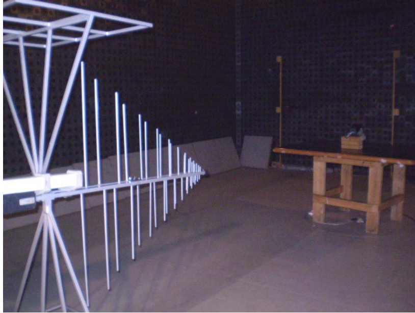
Photograph No.2 Radiated emissions measurement setup in the anechoic chamber in 30 – 1000 MHz
