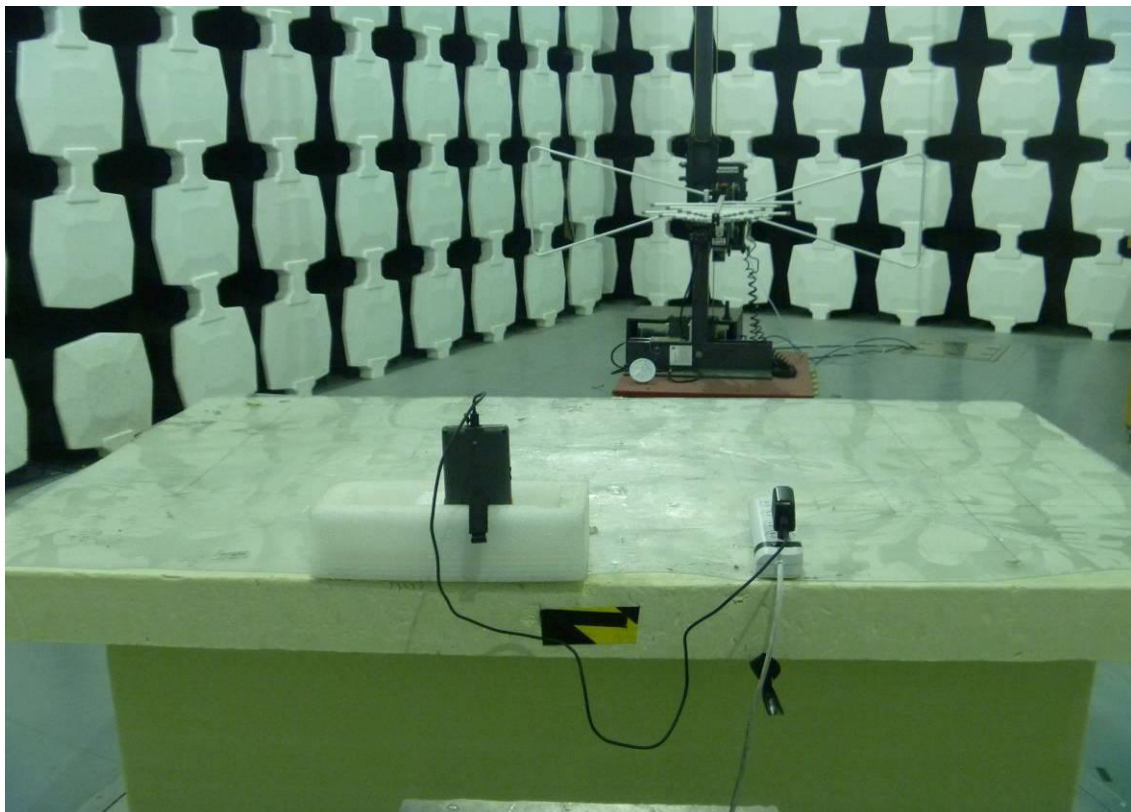
Radiated Measurement Setup (From 30MHz to 1GHz)
