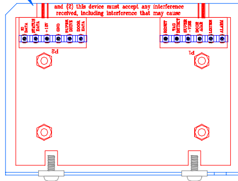
Top View of Mounting Plate with Receiver in Place
