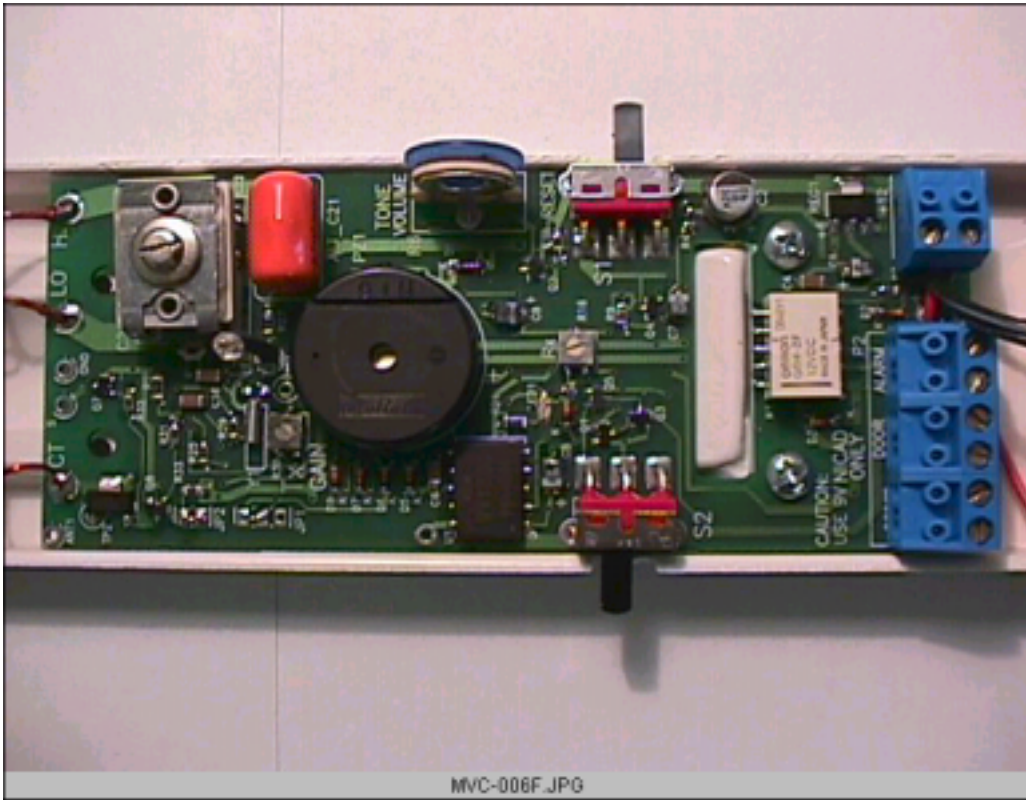
Innovative Control - Transceiver PCB / Component Side
