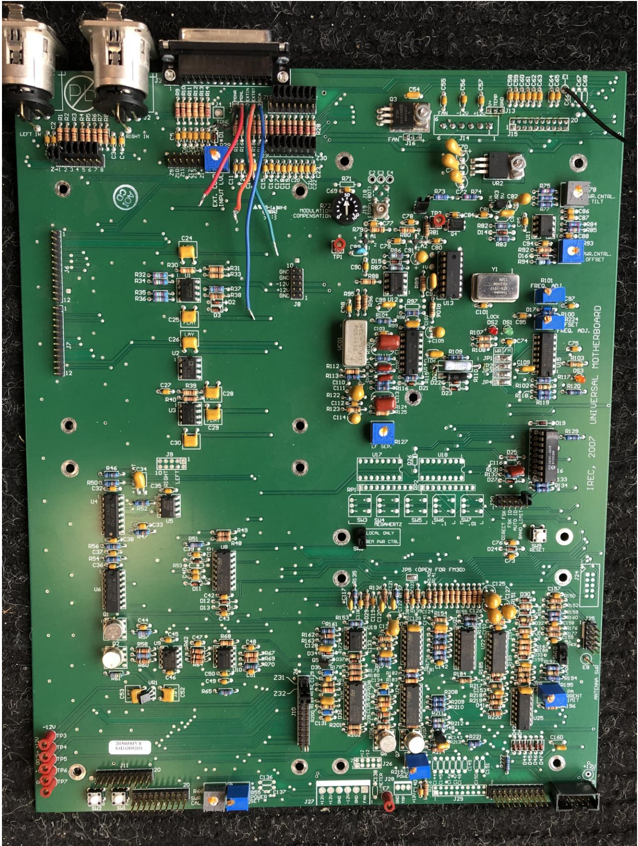
Mother board w/ exciter - front
