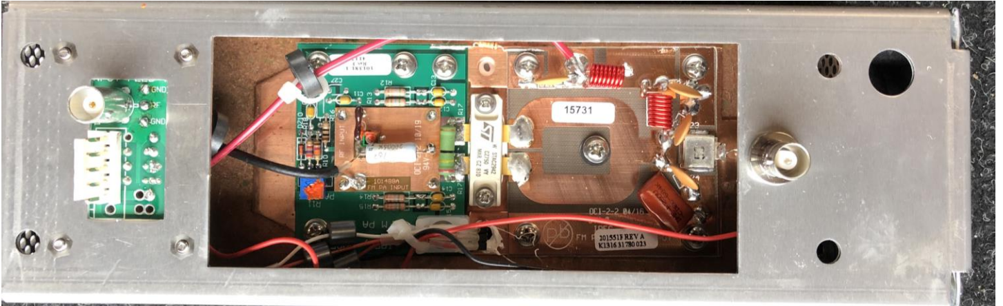
PA Module – attaches to the back of unit
