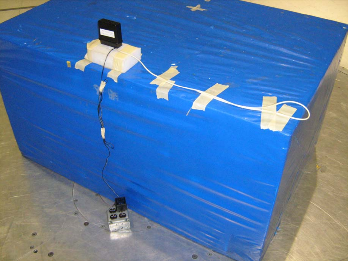
Figure 1 Test setup for Radiated Emissions
