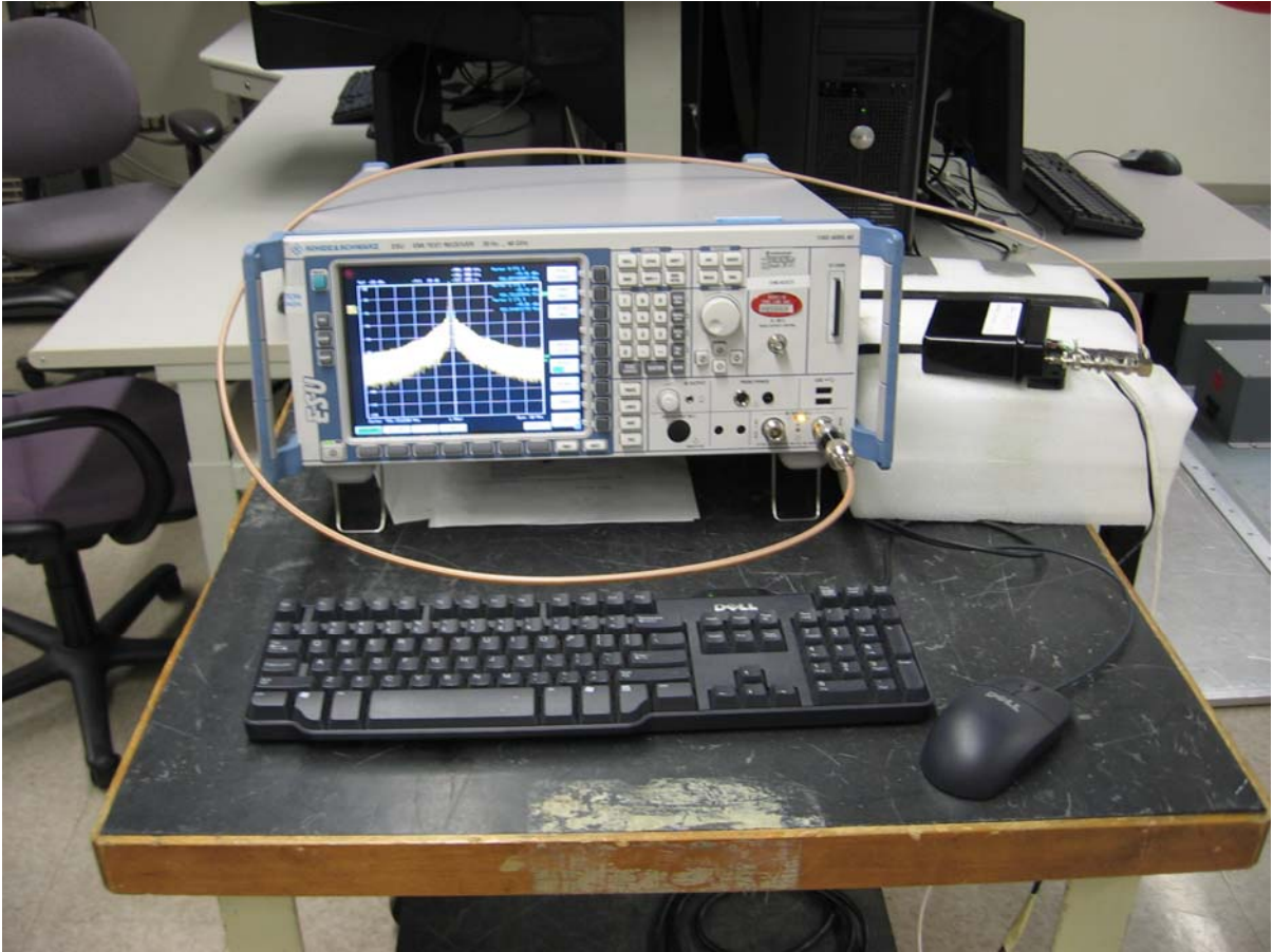
Figure 2 Test Setup for Occupied Bandwidth
