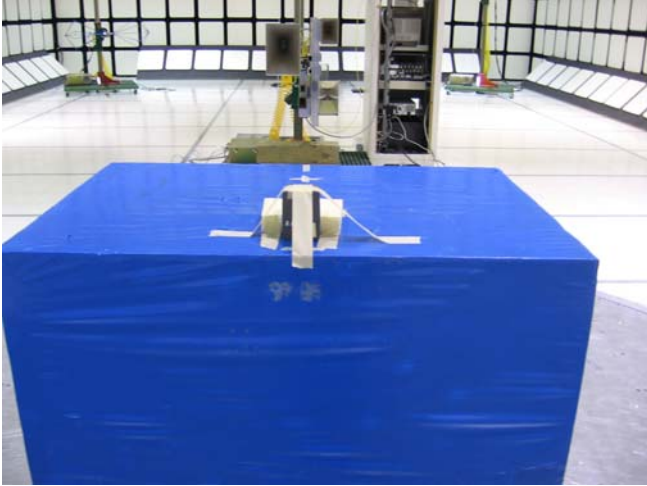
Radiated Emissions Setup
