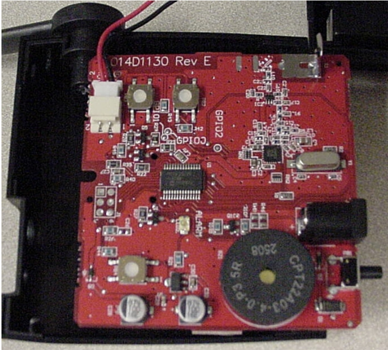
PCB – Component Side
