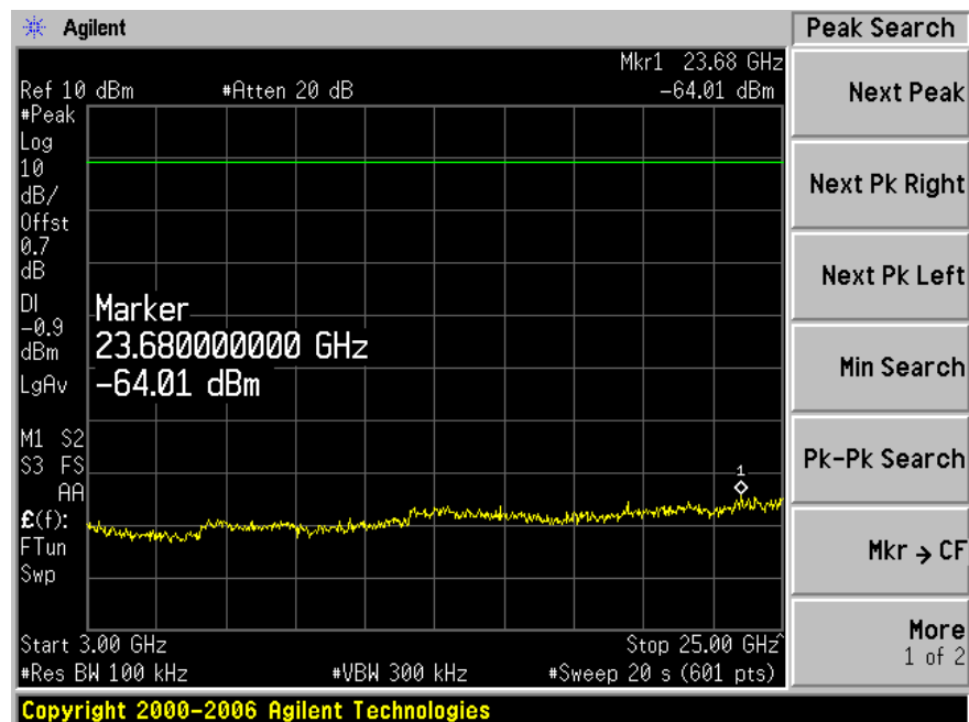
Plot 3-2: 3.0 to 25.0 GHz
