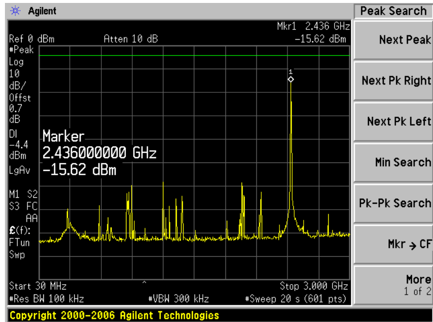
Plot 2-1: 30 MHz to 3.0 GHz
