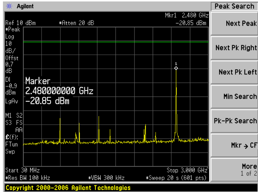
Plot 3-1: 30 MHz to 3.0 GHz
