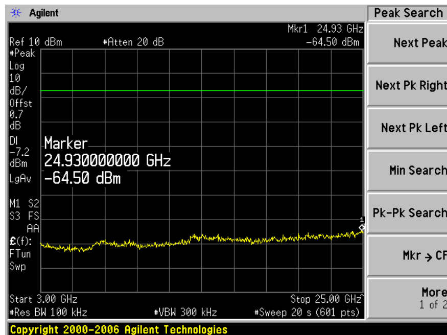
Plot 1-2: 3.0 to 25.0 GHz
