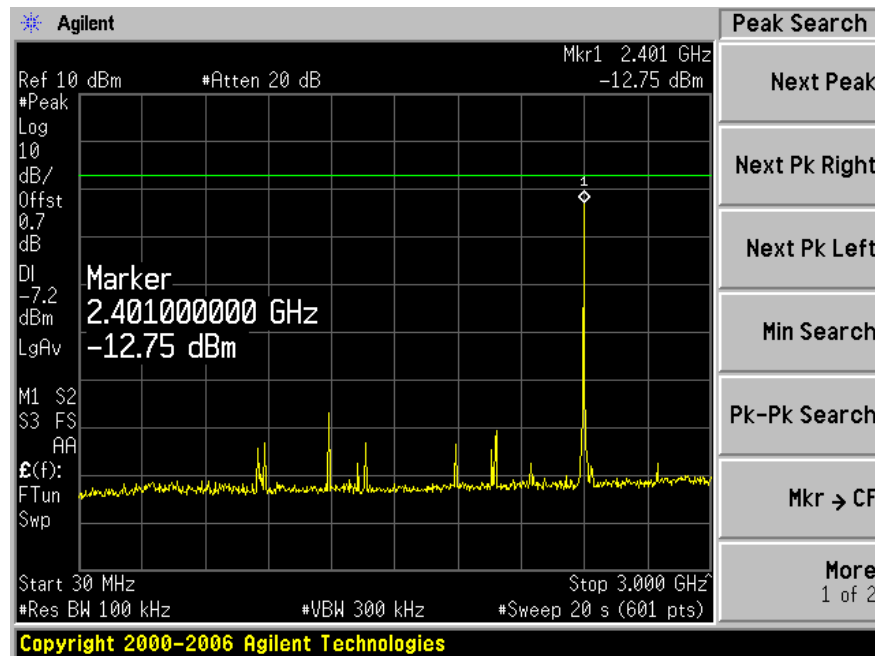
Plot 1-1: 30 MHz to 3.0 GHz
