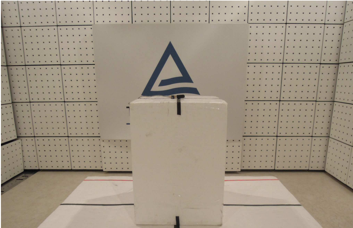
Photograph 1: Set-up for Radiated Emissions (Front View)
