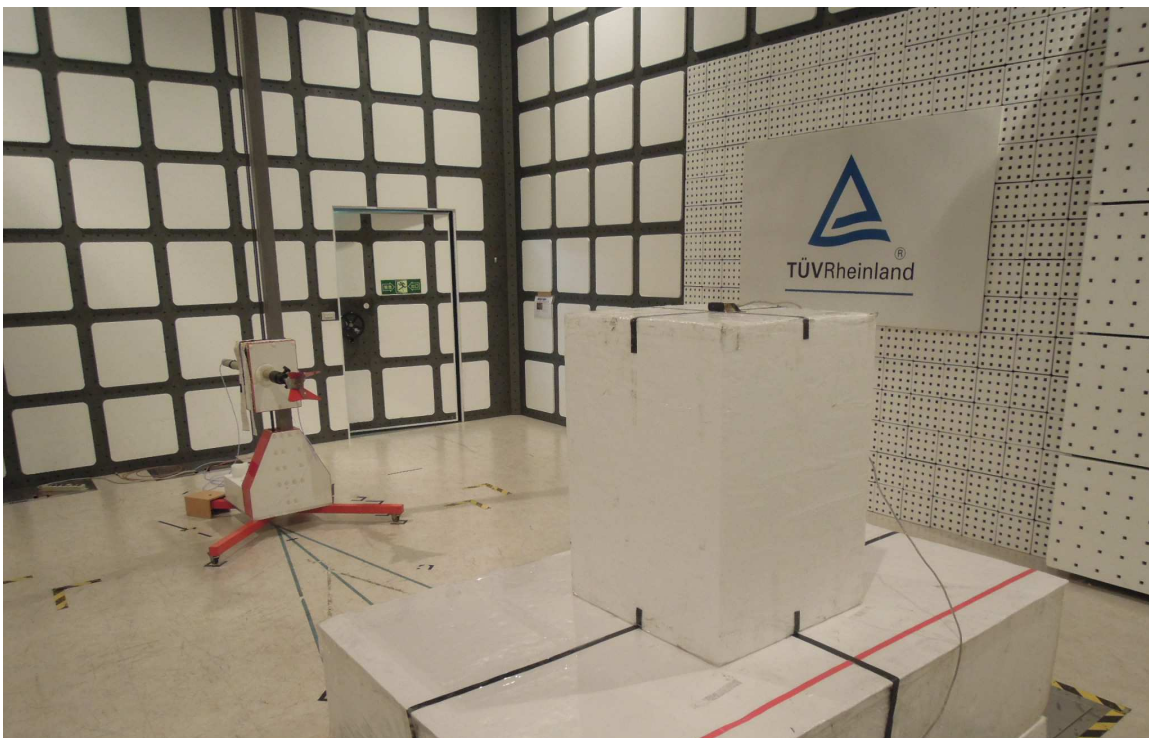
Photograph 3: Set-up for Radiated Emissions (Back View 2 TX)
