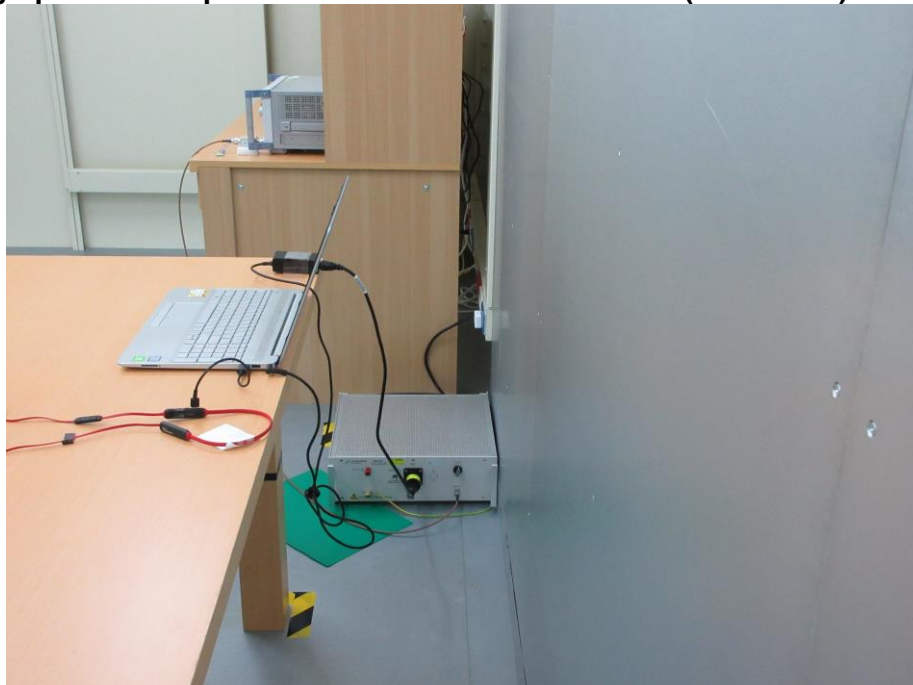
Photograph 10: Set-up for Mains Conducted Emissions (Back View)
