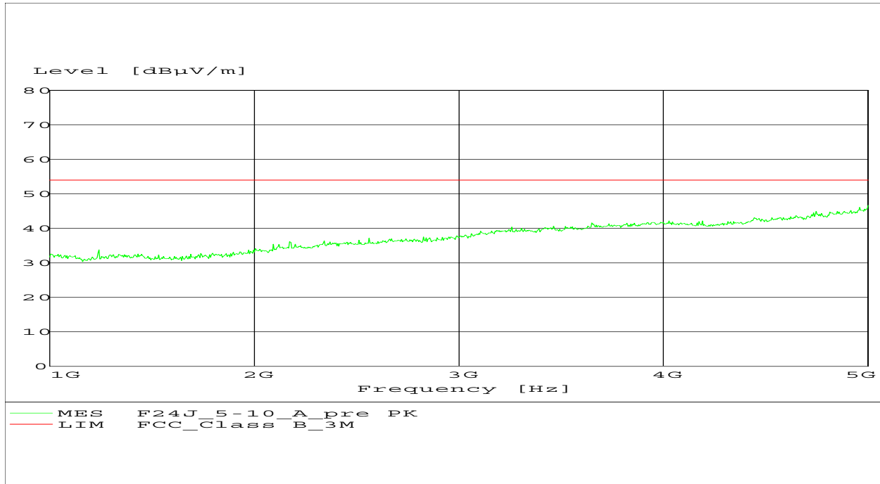
Plot 2 – Radiated Emissions – 1GHz to 5GHz
