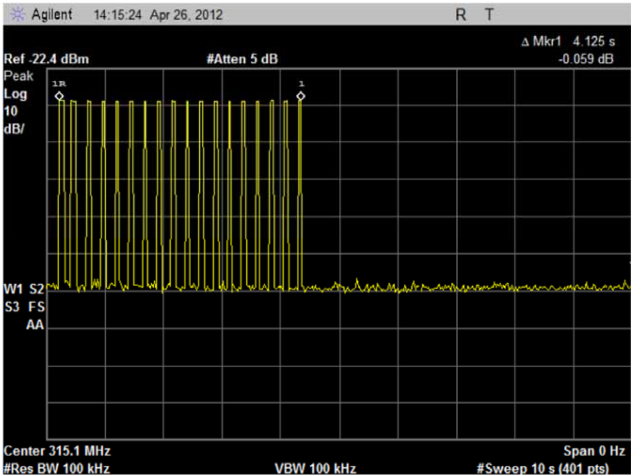
Plot 2 – Deactivation Time – Continuous Transmit Mode
