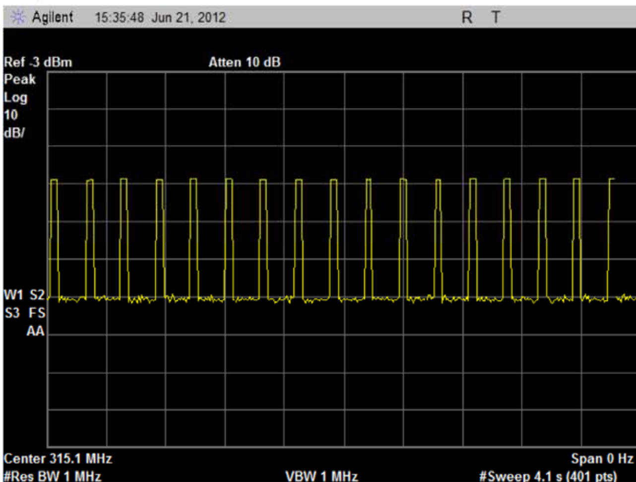
Plot 4 – Duty Cycle
