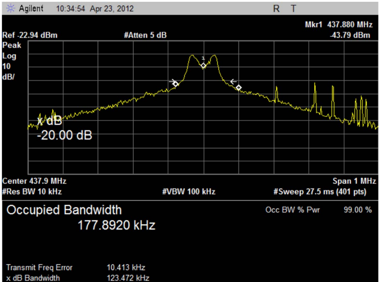
Plot 1 – 20dB BW FSK Modulation & 99% Occupied BW (For IC Only)
