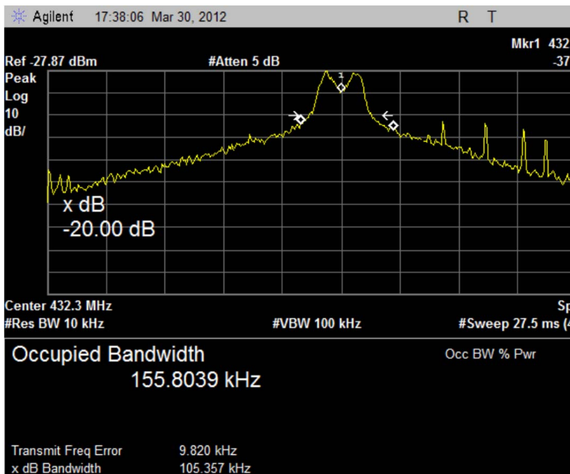
Plot 1 – 20dB BW FSK Modulation & 99% Occupied BW (For IC Only)
