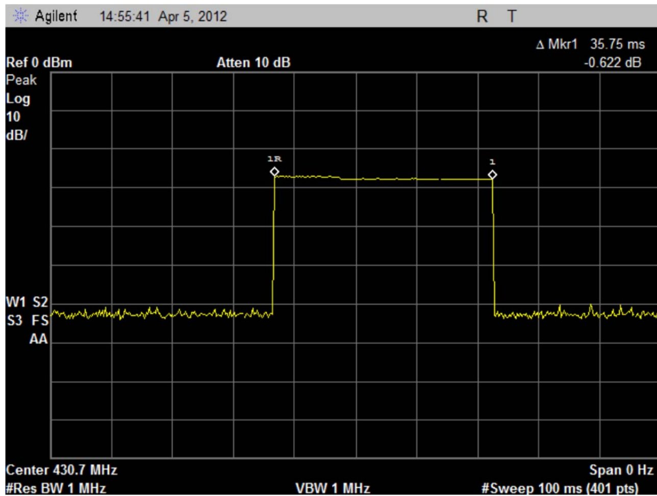
Plot 3 – Duty Cycle – On Time
