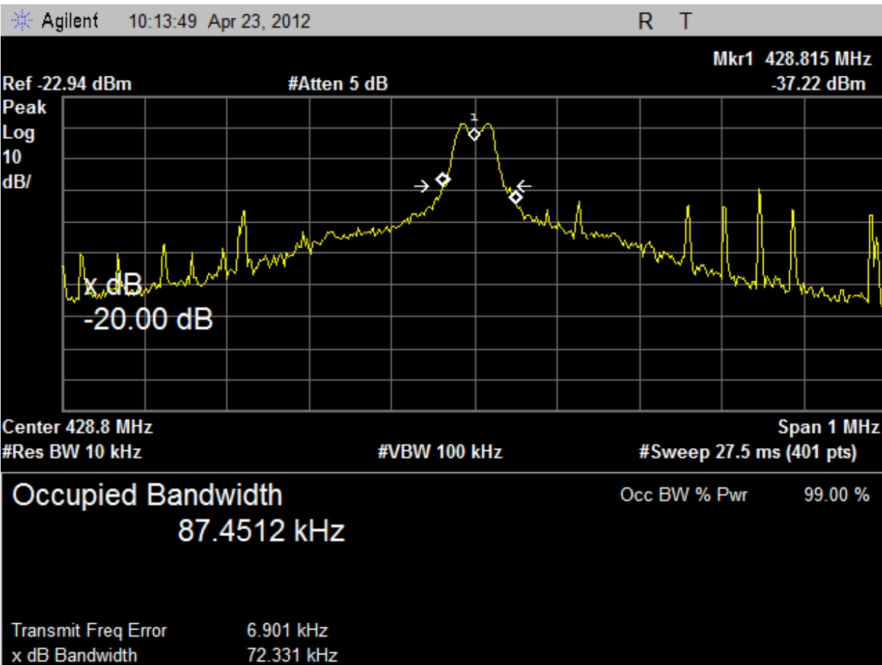
Plot 3 – 20dB BW FSK Modulation & 99% Occupied BW (For IC Only)
