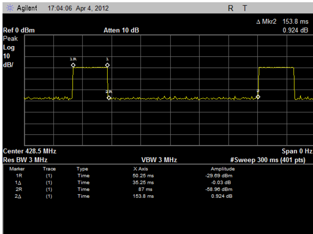
Plot 7 – Duty Cycle – On/Off Time
