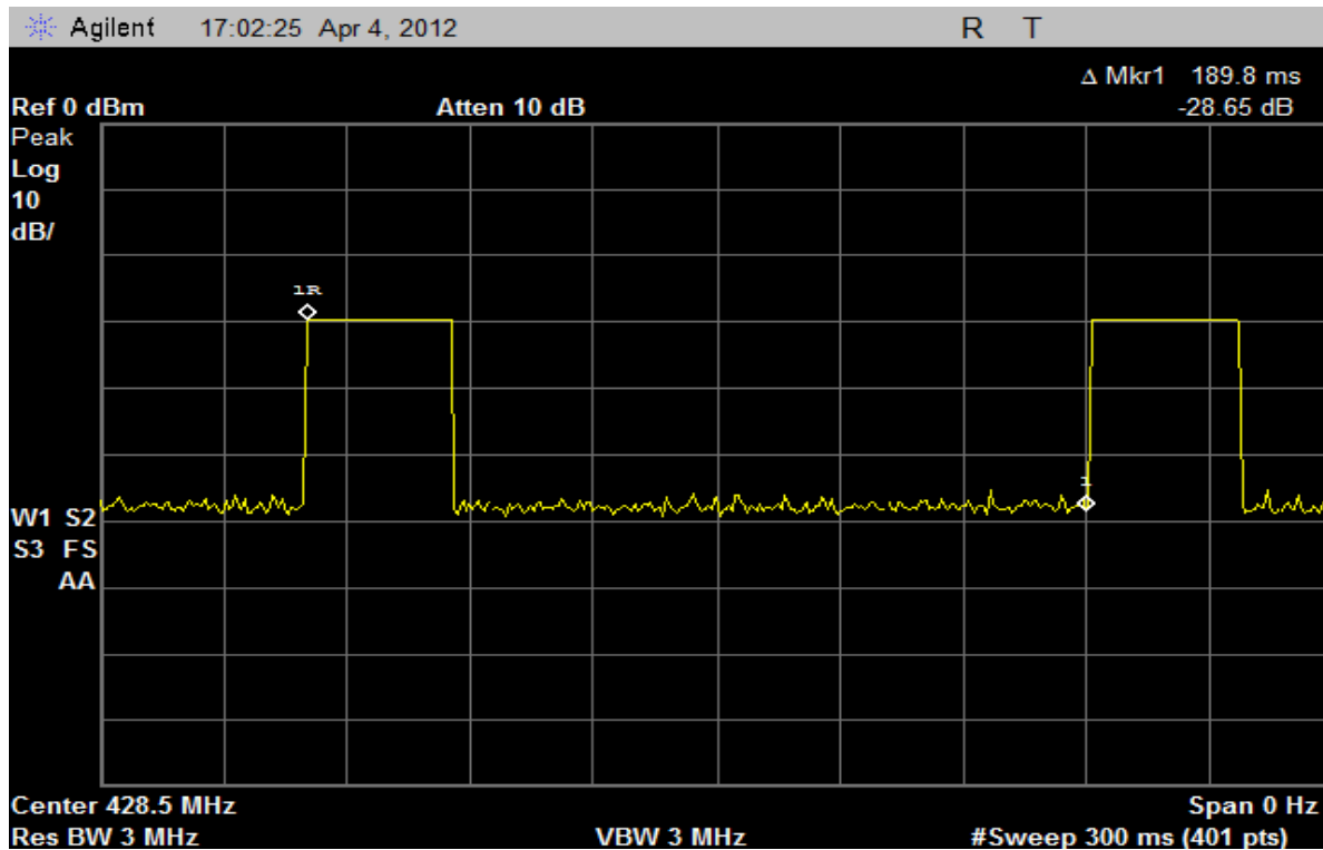
Plot 6 – Duty Cycle - Period
