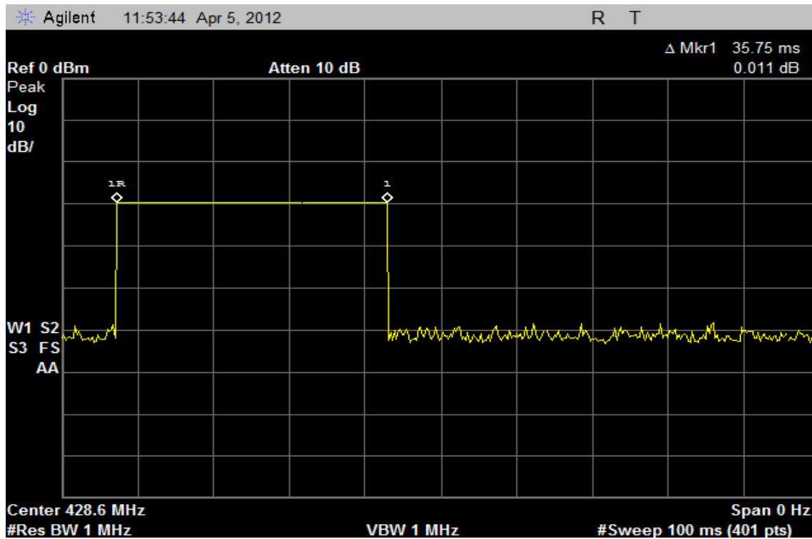
Plot 5 –Duty Cycle - On Time
