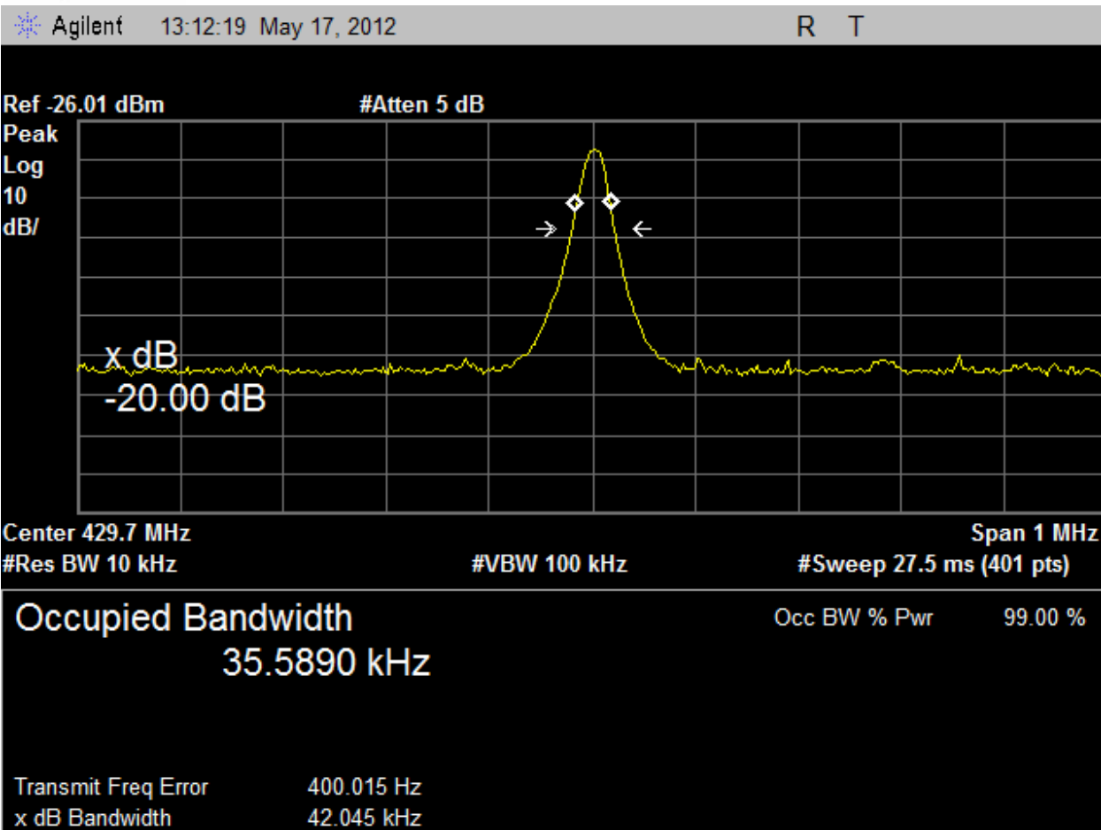
Plot 2 – 20dB BW FSK Modulation & 99% Occupied BW (For IC Only) – Middle Channel
