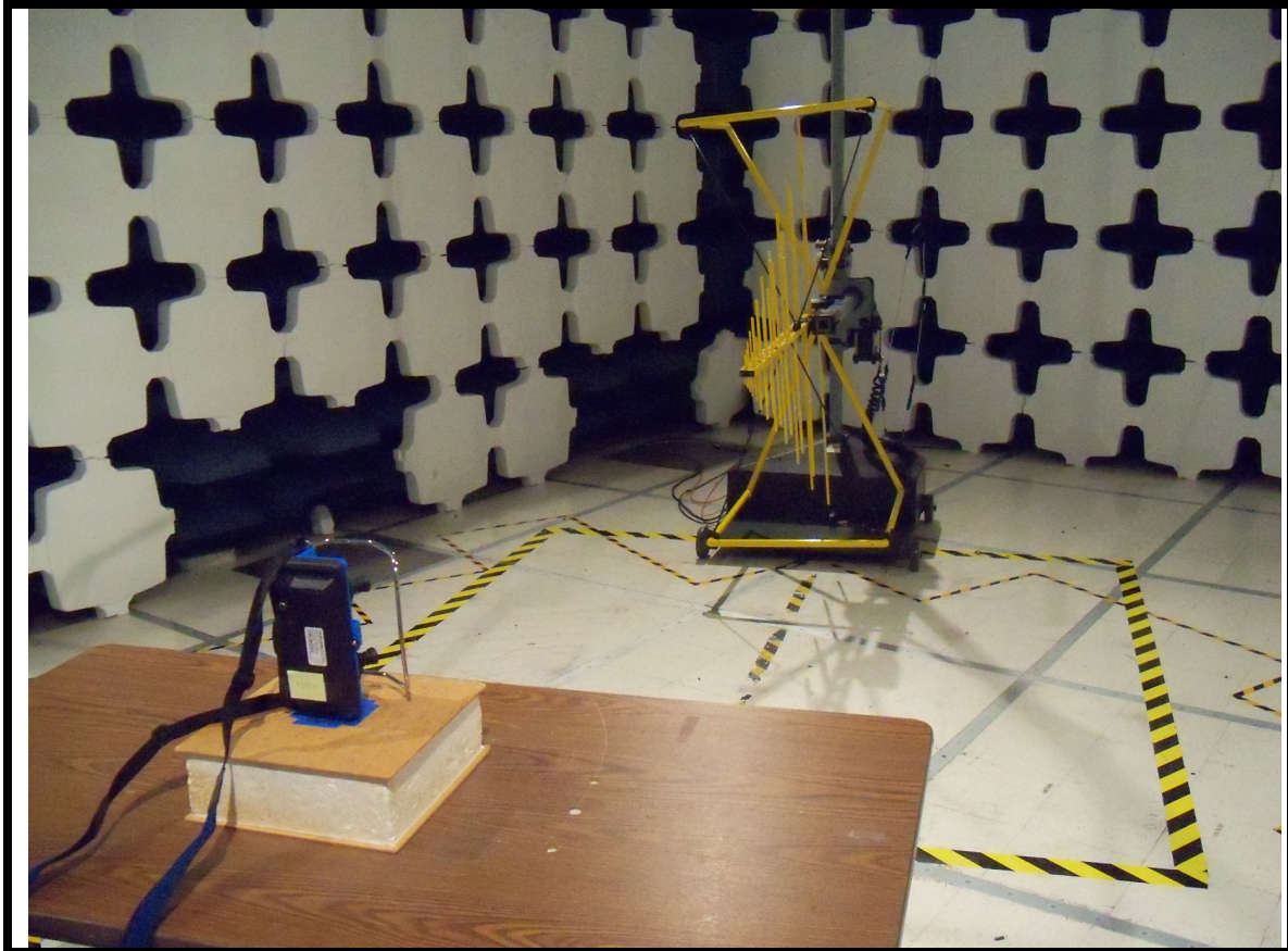
Test Setup Photo – F22 J
