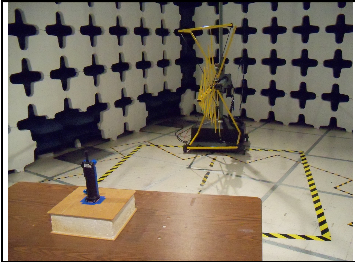
Test Setup Photo – F22 12D
