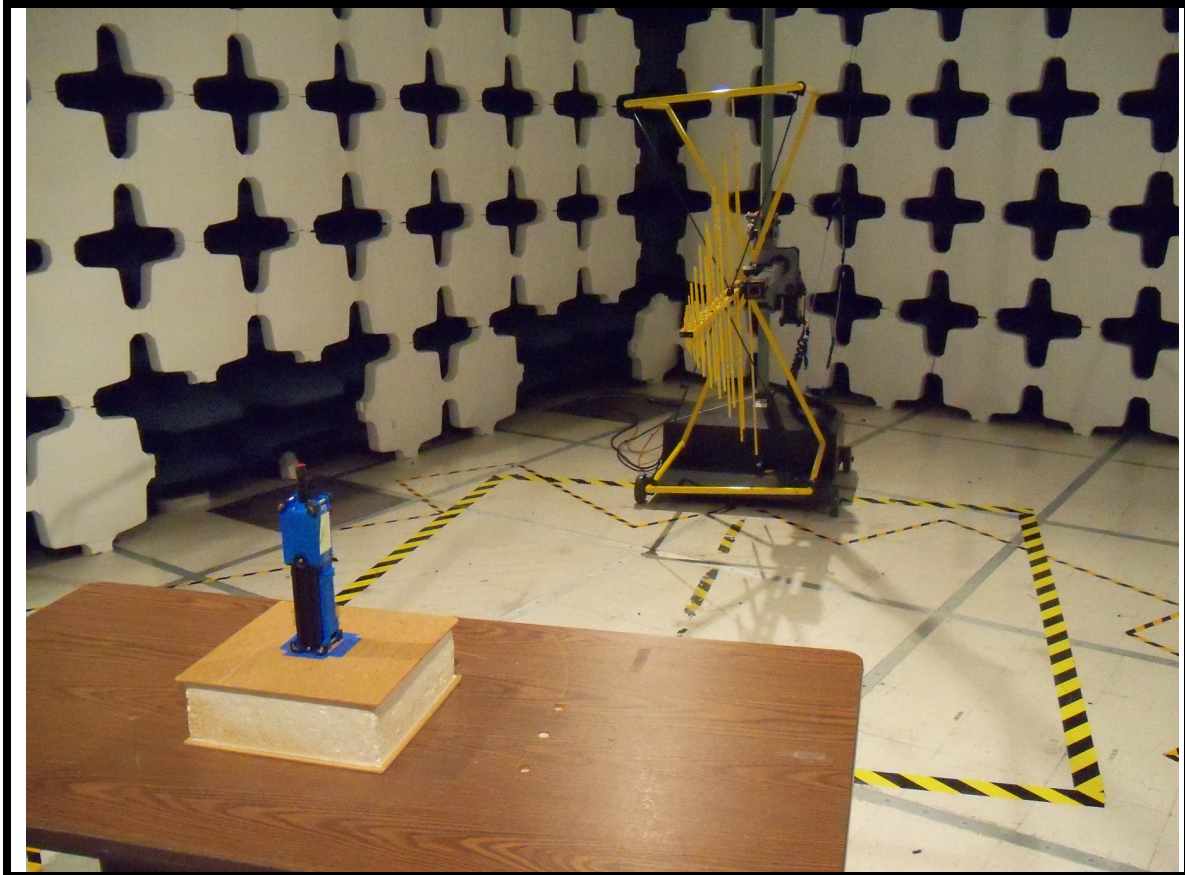
Test Setup Photo – F22 10D
