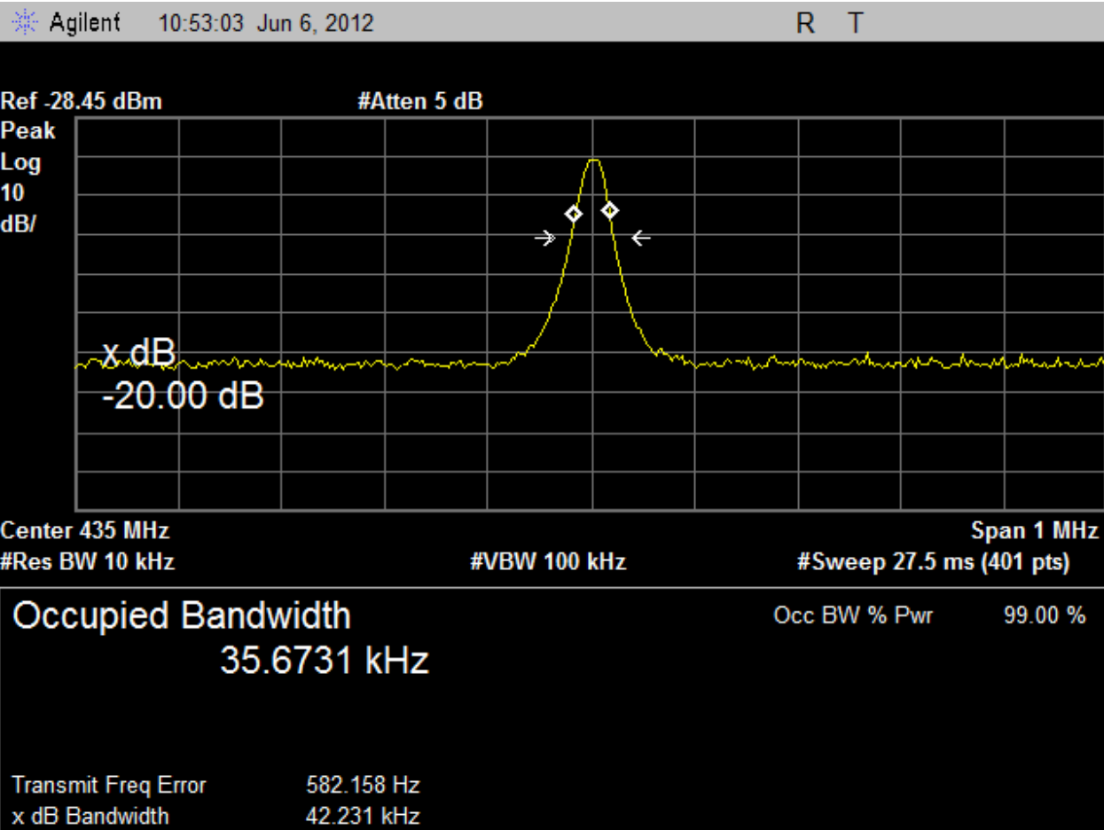
Plot 3 – 20dB BW FSK Modulation & 99% Occupied BW (For IC Only) – High Channel
