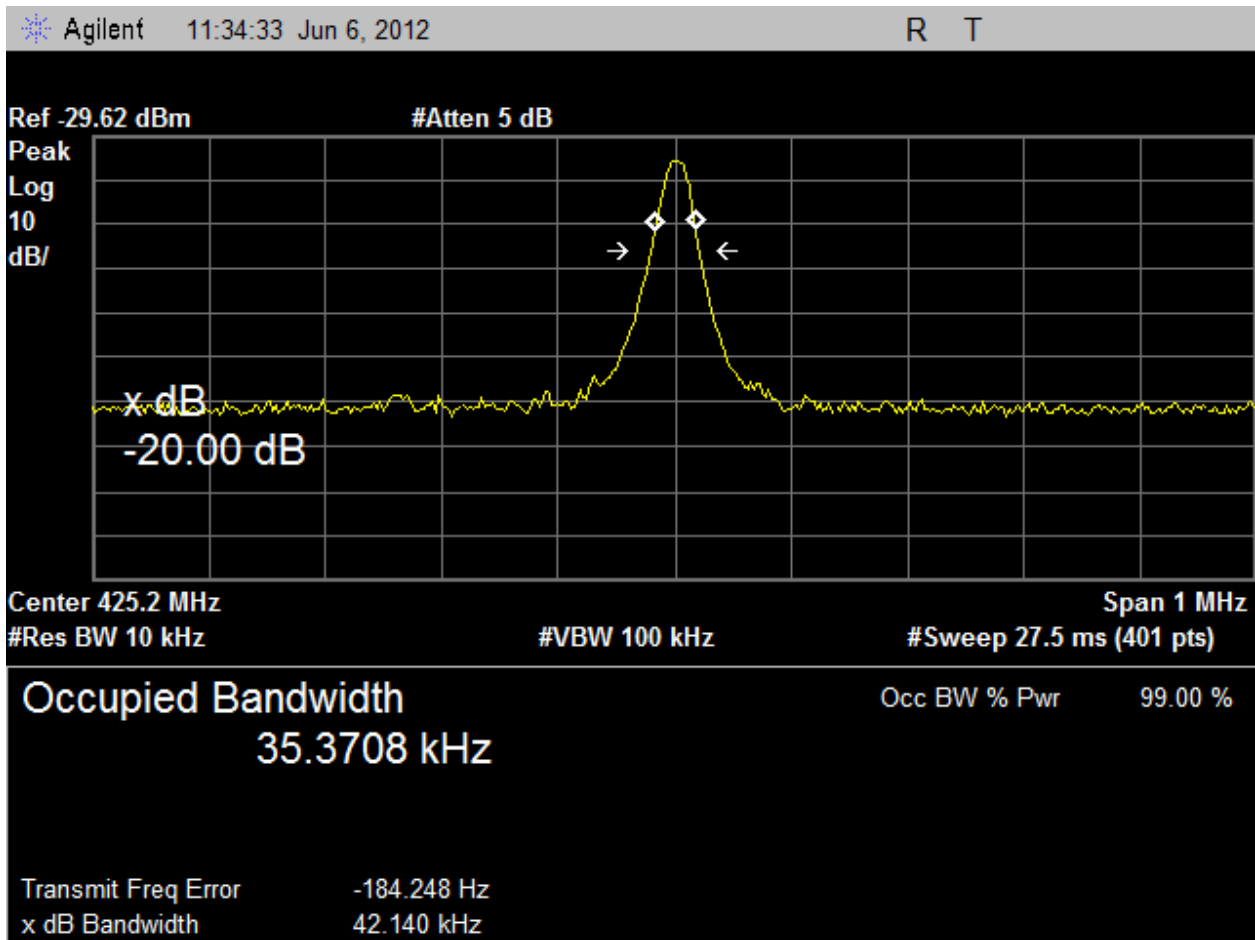
Plot 1 – 20dB BW FSK Modulation & 99% Occupied BW (For IC Only) – Low Channel
