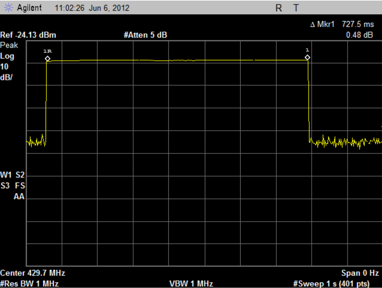
Plot 5 – Duty Cycle
