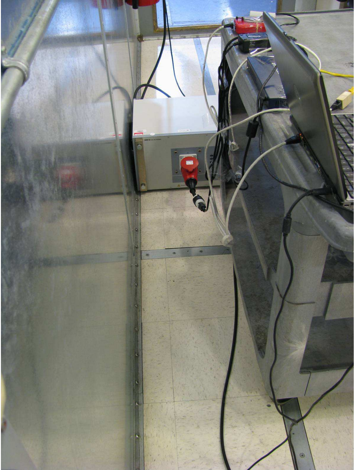
Conducted Power Port Emissions (Back)
