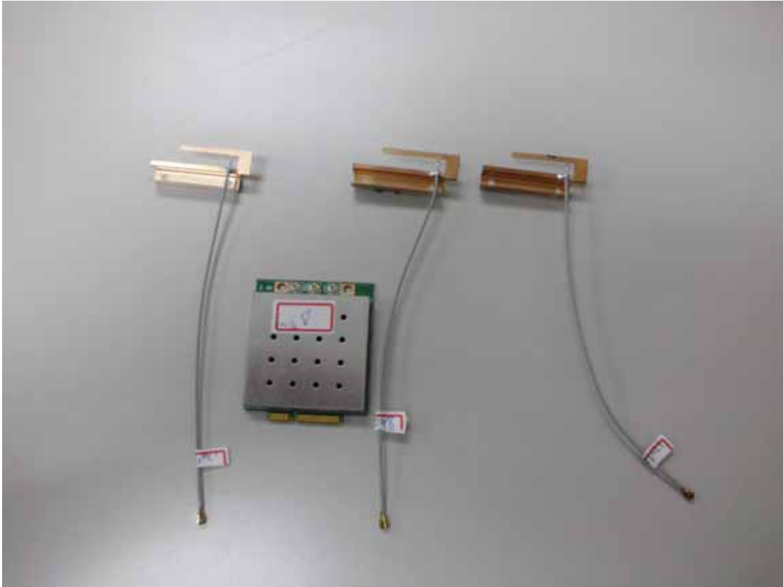
Figure 2 2.4GHz 802.11n 3T3R wifi module (Front View)
