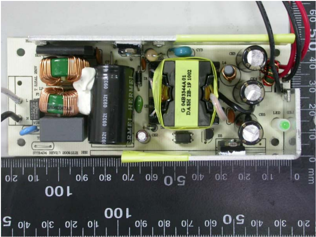
17. Front view of PCB6
