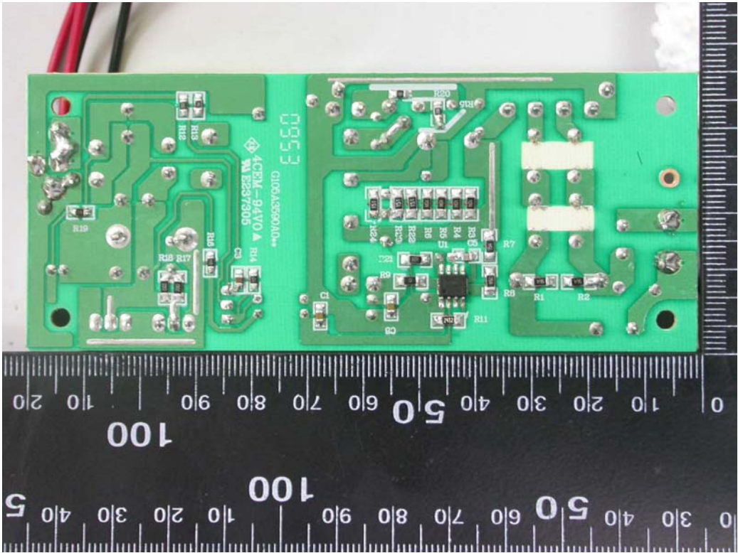
18. Rear view of PCB6
