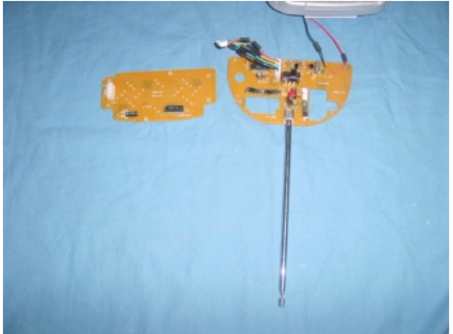
Figure 4 Main Board, Component Side
