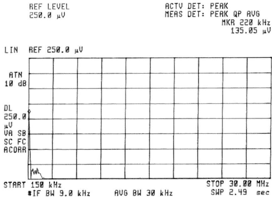
Figure 5.1.b Neutral Conducted-9V
