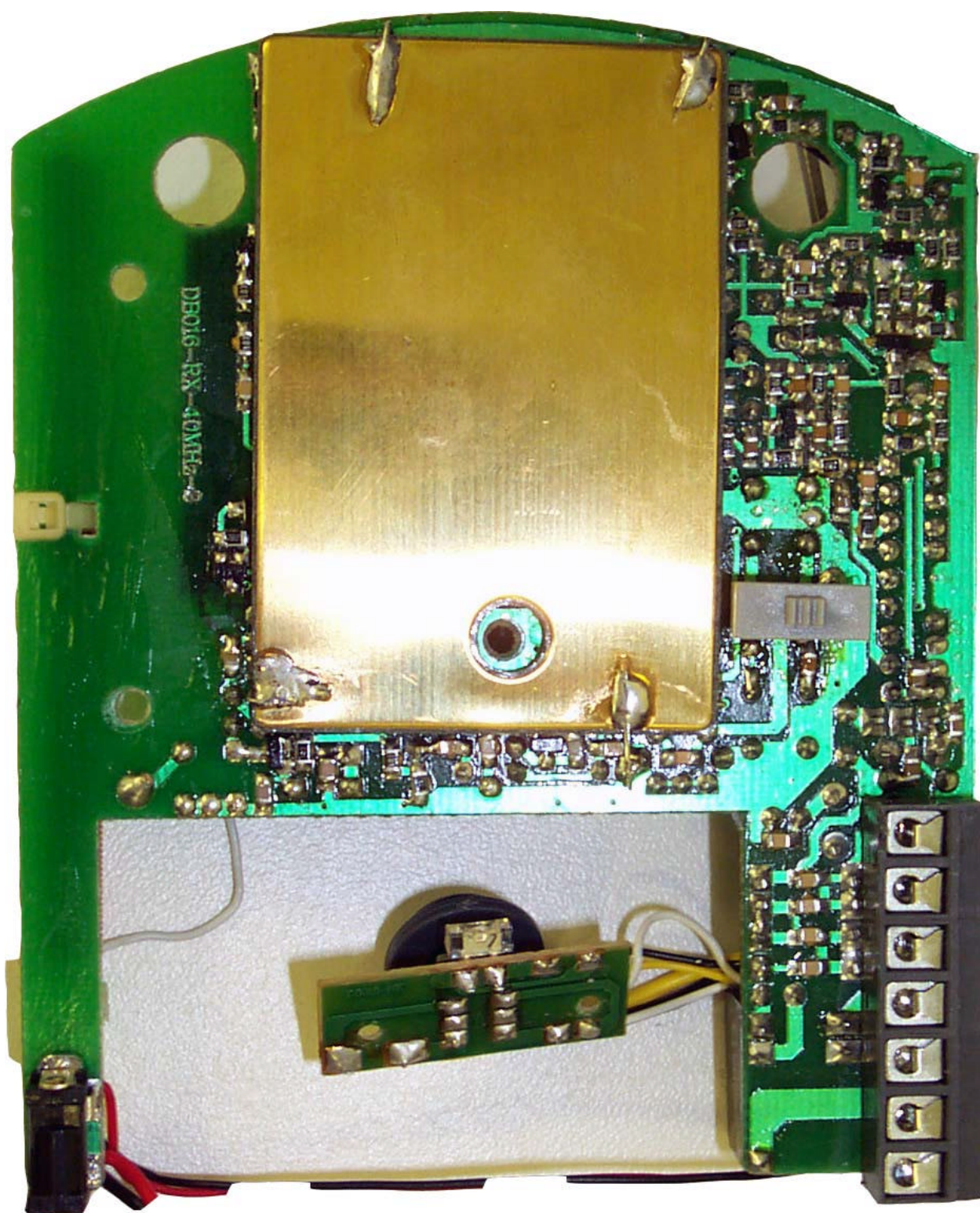
Foil Side
