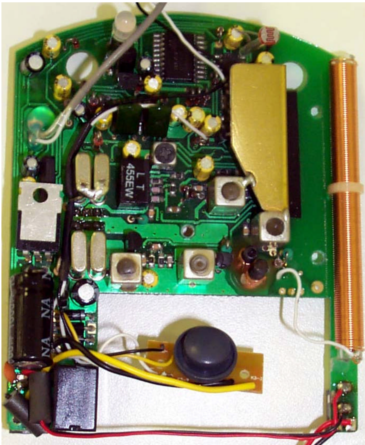
Component Side
