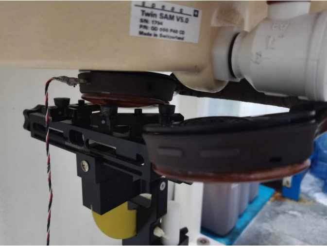
Fig-4.2 Front Side of EUT with 0 cm Gap (Head Mode)
