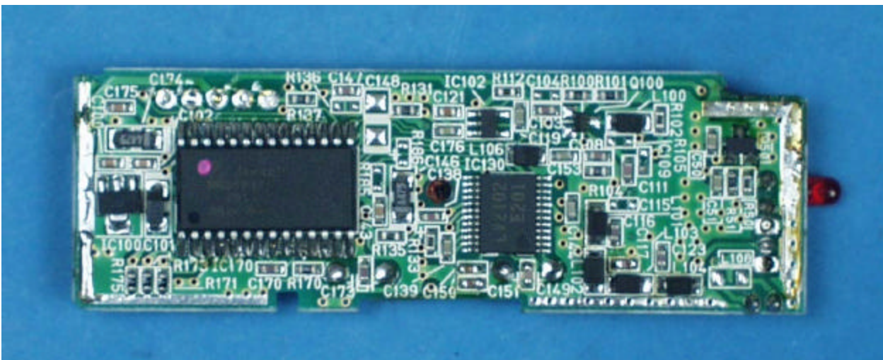
RF Board, Side 1 w/o Shield
