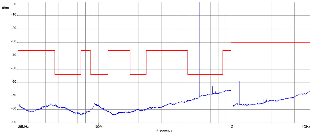
Plot 4: 580.000 MHz, spurious emissions, 25 MHz – 4 GHz
