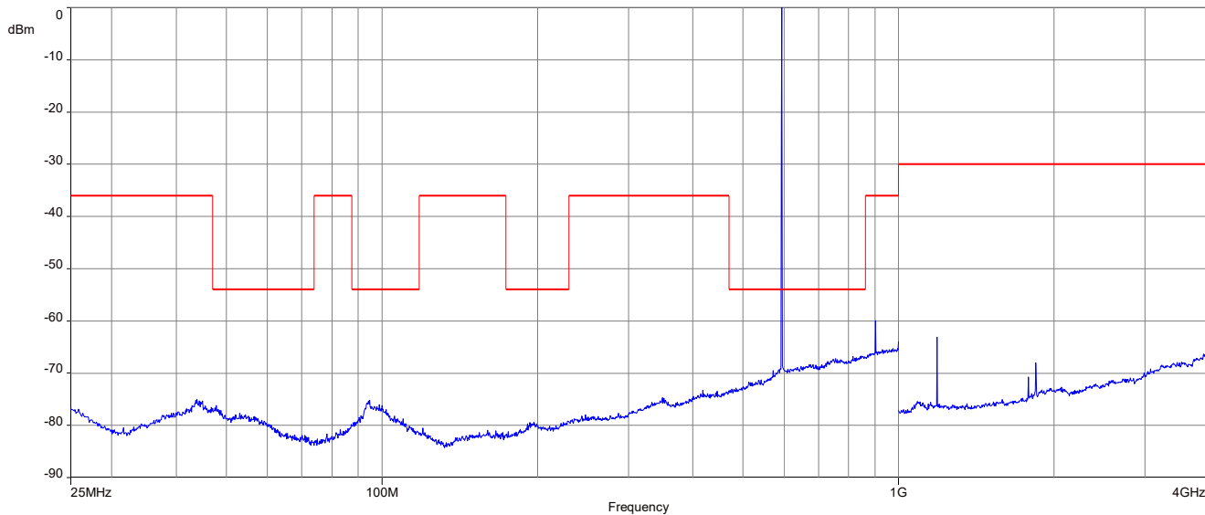
Plot 5: 594.000 MHz, spurious emissions, 25 MHz – 4 GHz
