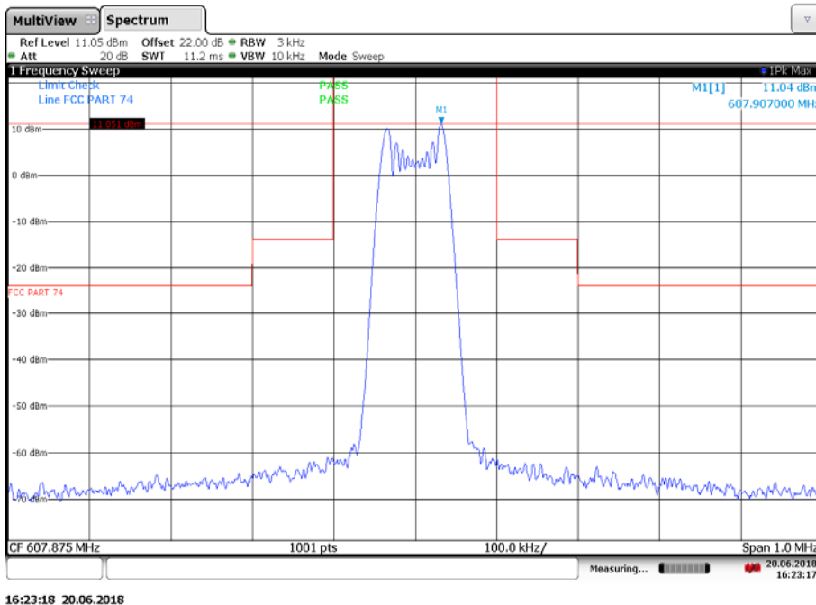
Plot 6: 607.875 MHz, spectrum mask
