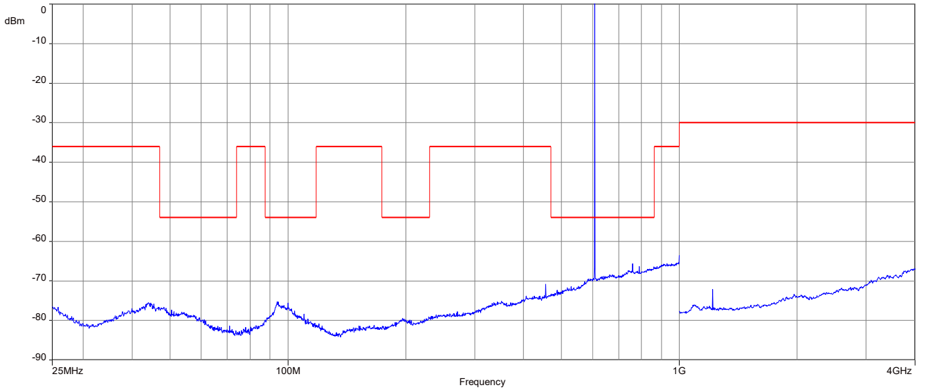
Plot 6: 607.875 MHz, spurious emissions, 25 MHz – 4 GHz
