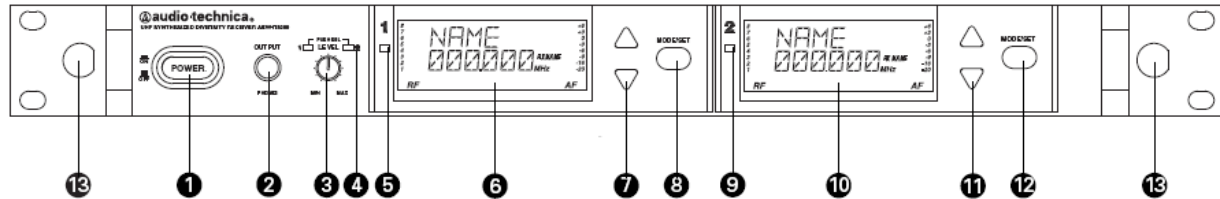
Figure C AEW-R5200 Receiver Front Panel
