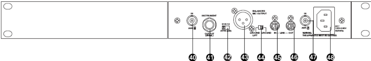
Figure F AEW-R4100 Receiver Rear Panel
