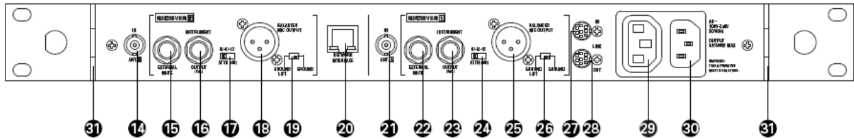
Figure D AEW-R5200 Receiver Rear Panel
