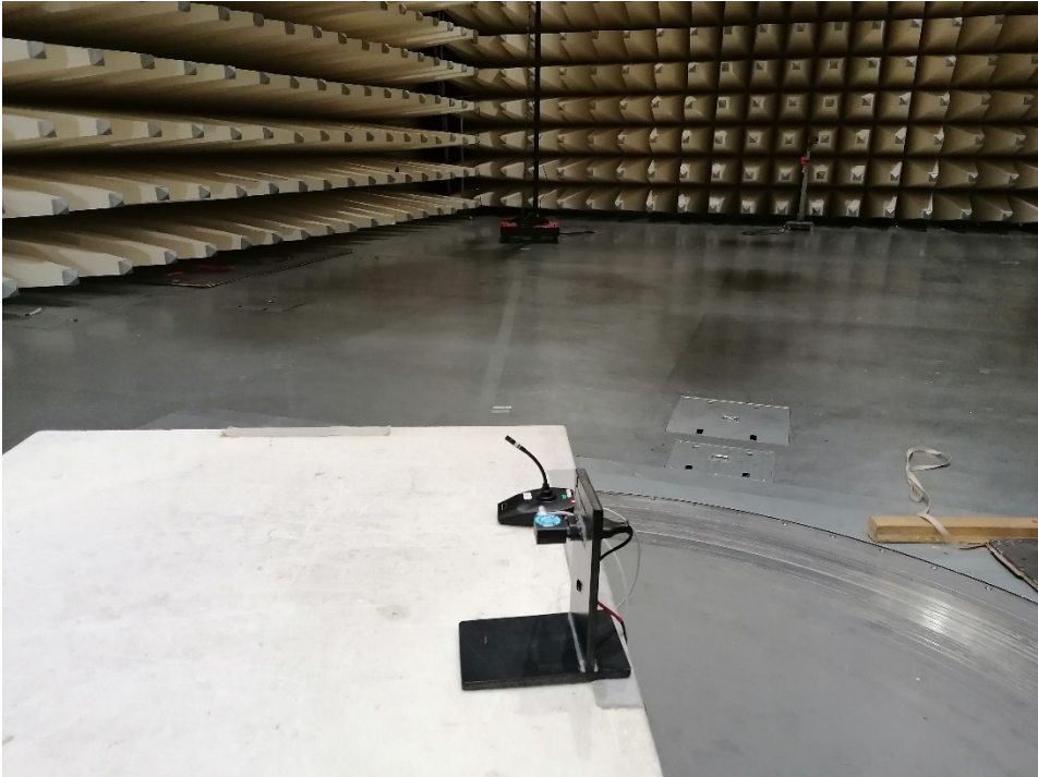
Photo 1: Radiated Emission
