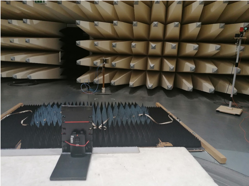
Photo 2: Radiated Emission
