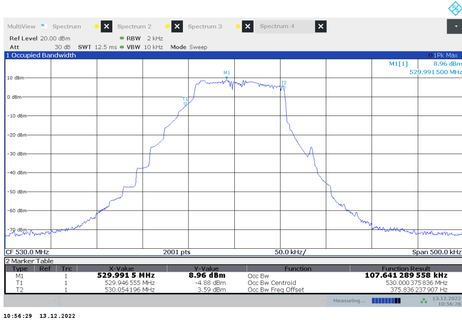
Plot 1: 530.000 MHz, max hold with frequency variation from 50 Hz to 15 kHz
