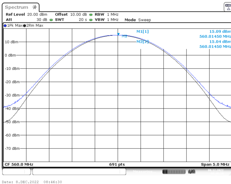
Plot 2: 560.000 MHz (modulated carrier)
