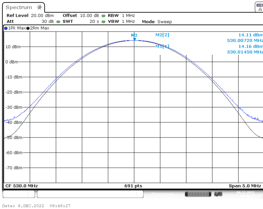
Plot 1: 530.000 MHz (modulated carrier)
