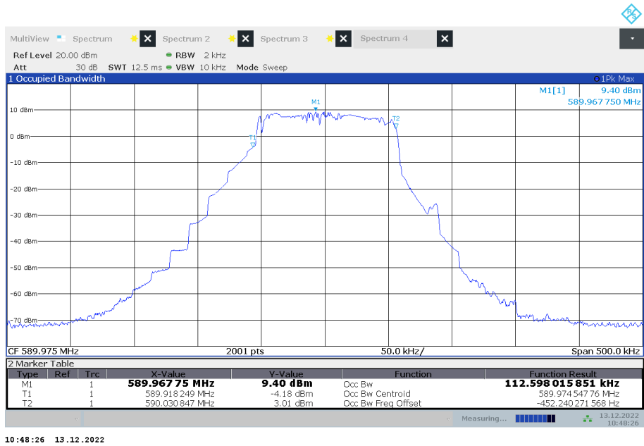
Plot 3: 589.975 MHz, max hold with frequency variation from 50 Hz to 15 kHz
