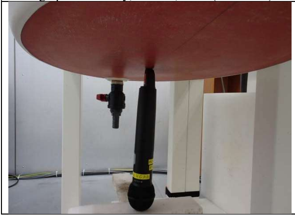
Photograph B10: Body, Bottom, 0mm (Side view)
