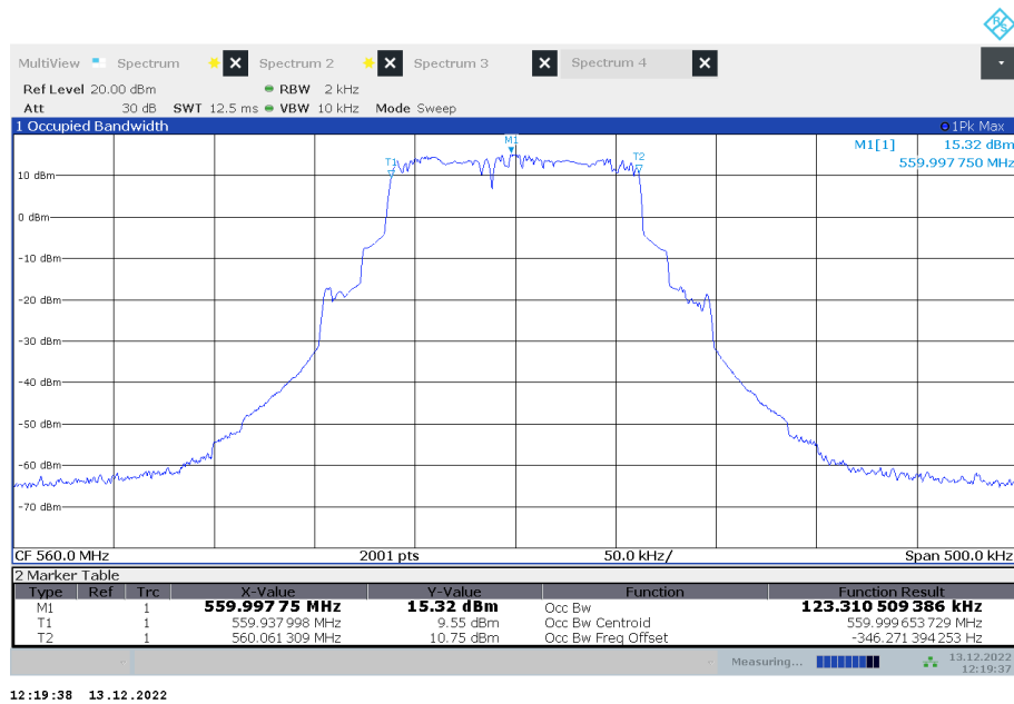
Plot 2: 560.000 MHz, max hold with frequency variation from 50 Hz to 15 kHz
