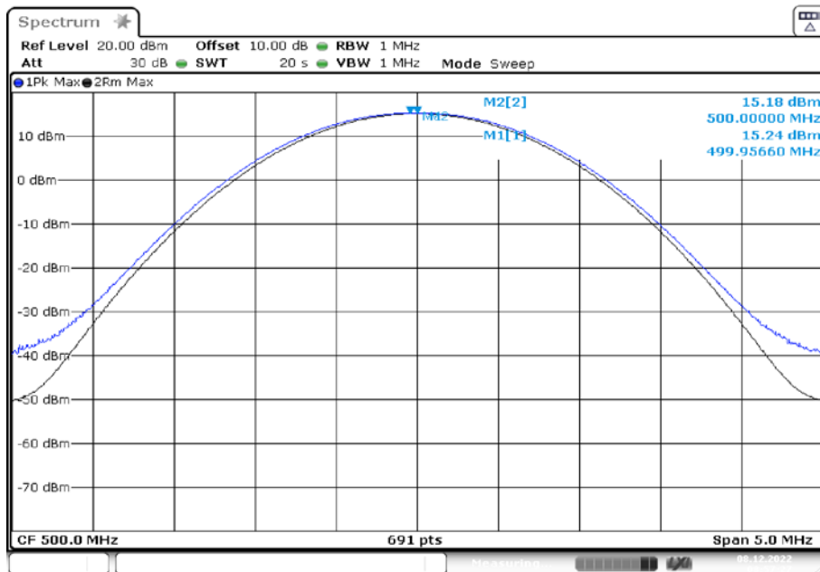
Plot 2: 500.000 MHz (modulated carrier)
