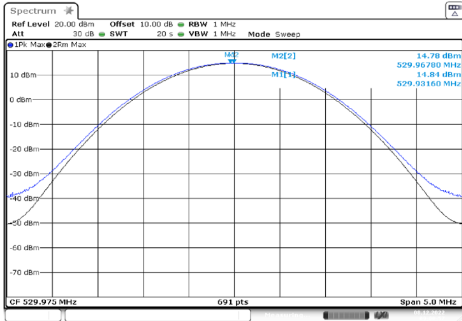
Plot 3: 529.975 MHz (modulated carrier)
