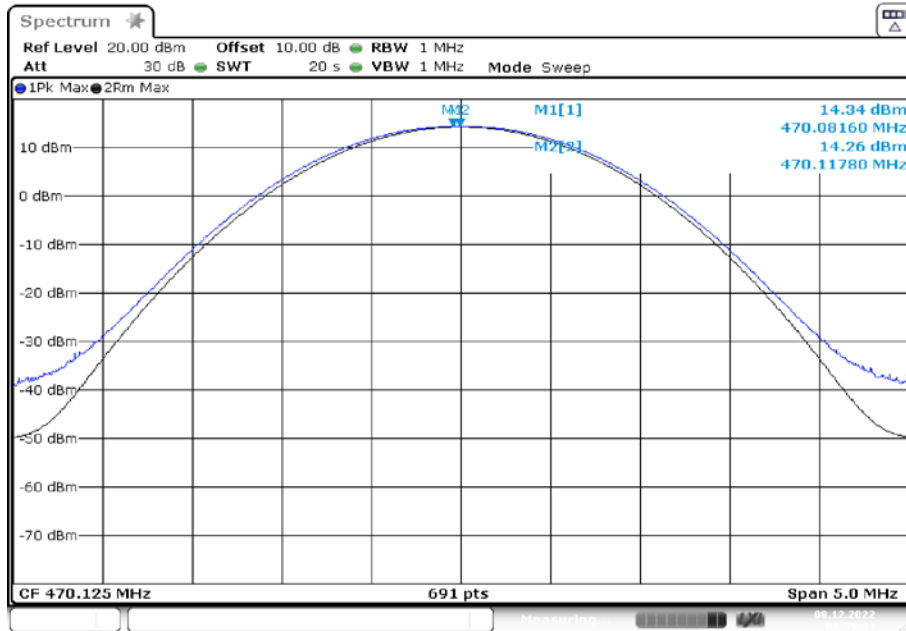
Plot 1: 470.125 MHz (modulated carrier)
