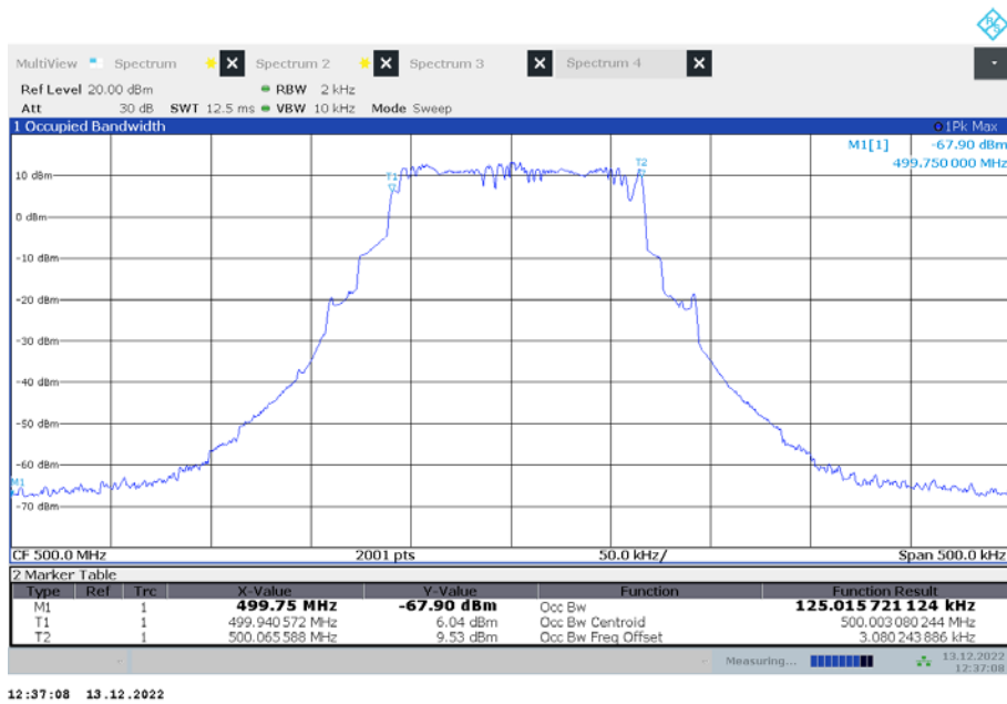
Plot 2: 500.000 MHz, max hold with frequency variation from 50 Hz to 15 kHz
