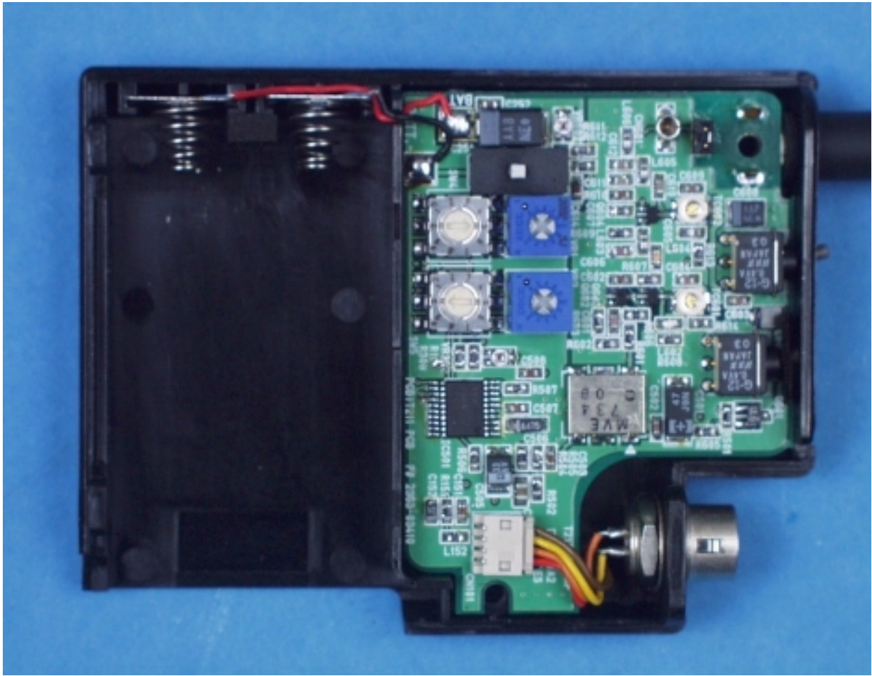
Circuit Board – Component Side
