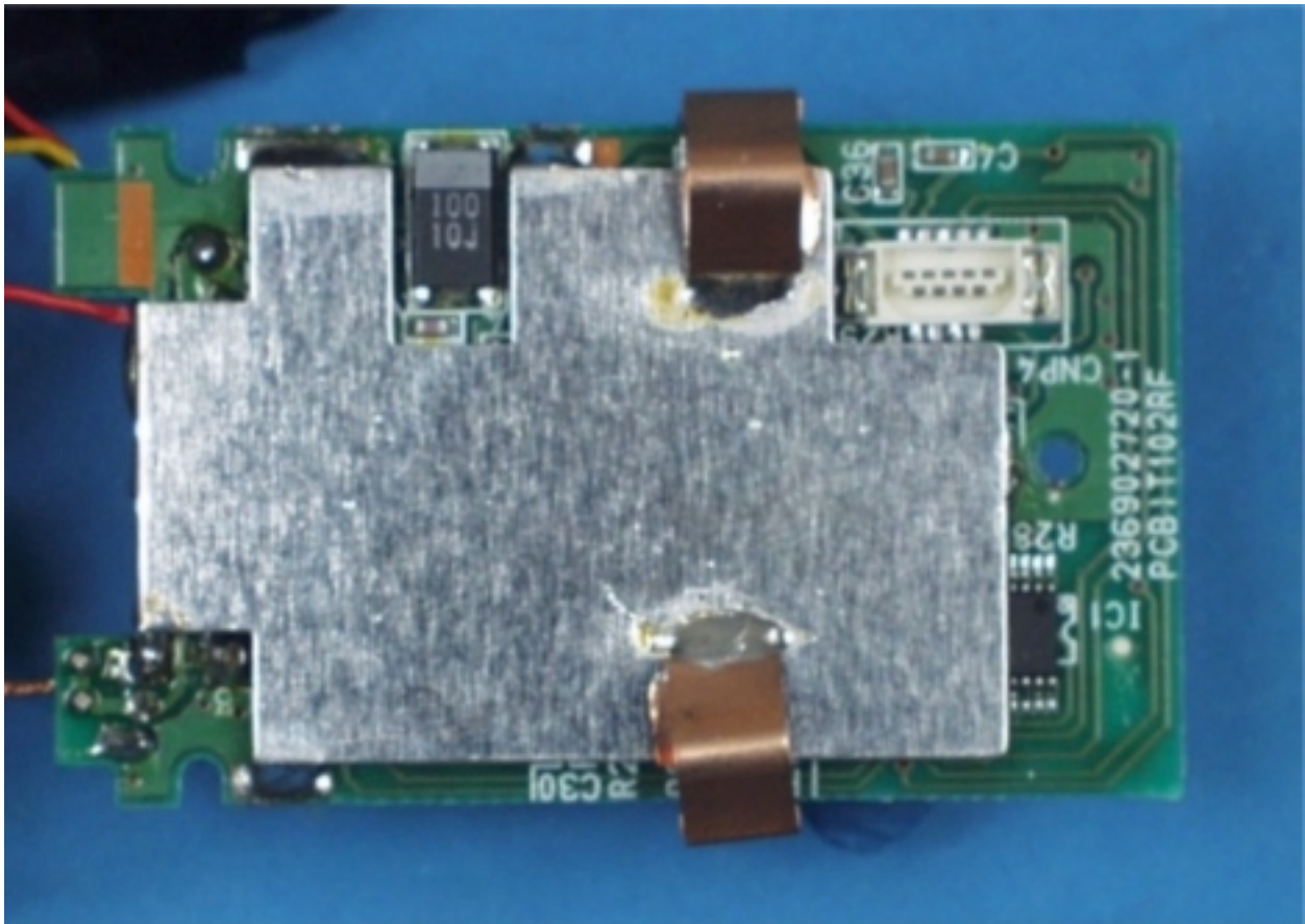
RF Bottom
