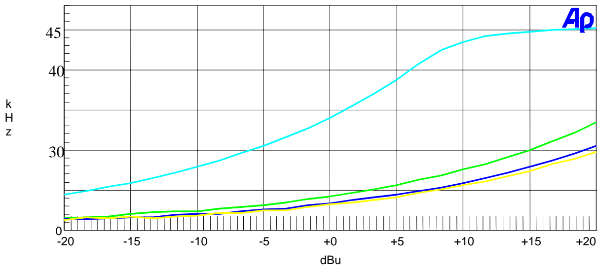
Modulation Limiting Plots: 15KHz (Cyan), 2.5KHz (Green), 1.0KHz (Blue), and 300Hz
