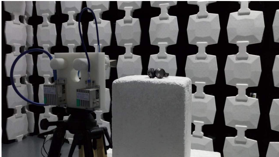
Description: Radiated Emission Test Setup (Above 18GHz)
