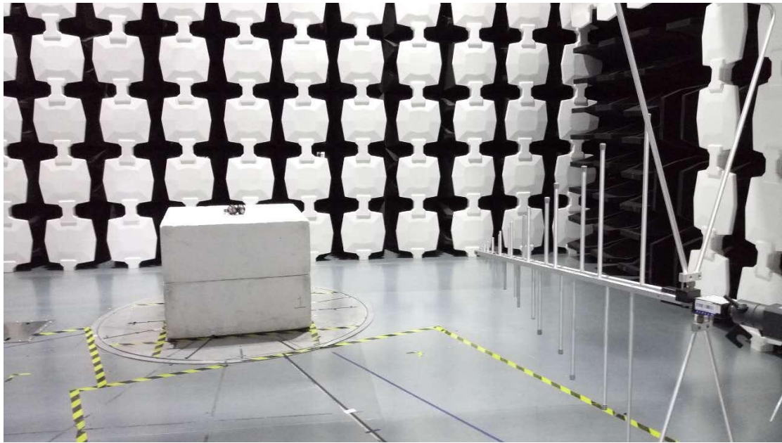
Description: Radiated Emission Test Setup (30-1000MHz)
