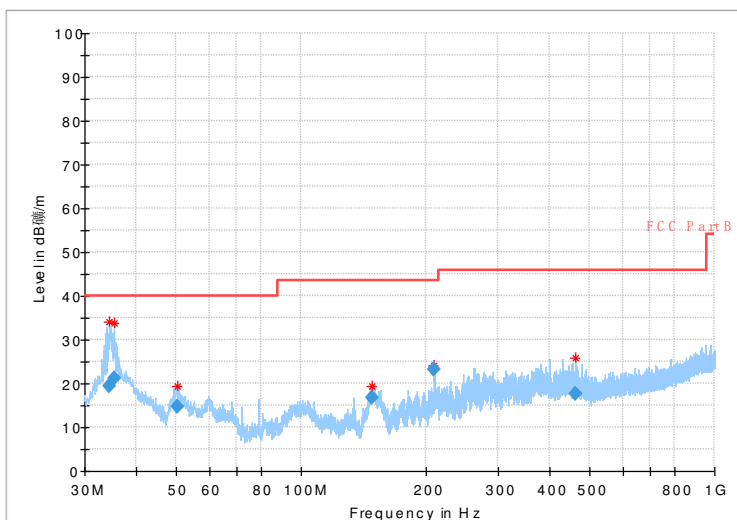
Fig.40 Radiated emission: GFSK, Ch78, 30MHz~1GHz
