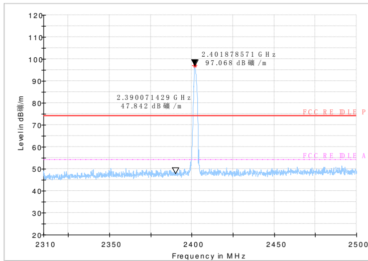
Fig.55 Radiated emission (Power): 8DPSK, low channel
