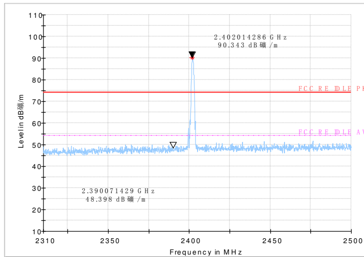
Fig.49 Radiated emission (Power): \pi/4 DQPSK, low channel
