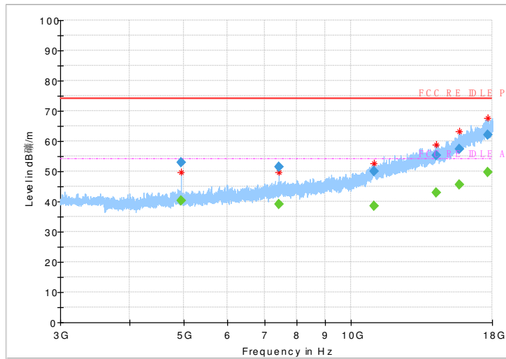
Fig.48 Radiated emission: \pi/4 DQPSK, Ch78, 3GHz~18GHz
