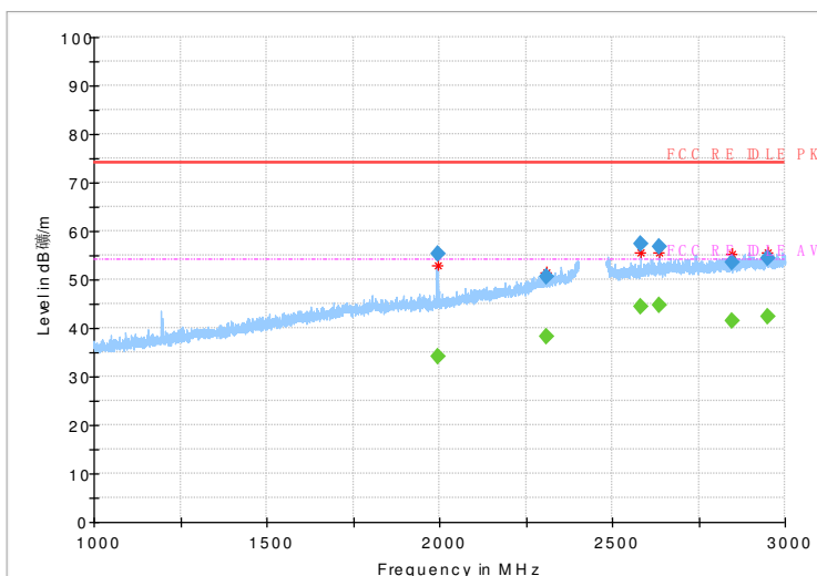
Fig.41 Radiated emission: GFSK, Ch78, 1GHz~3GHz
