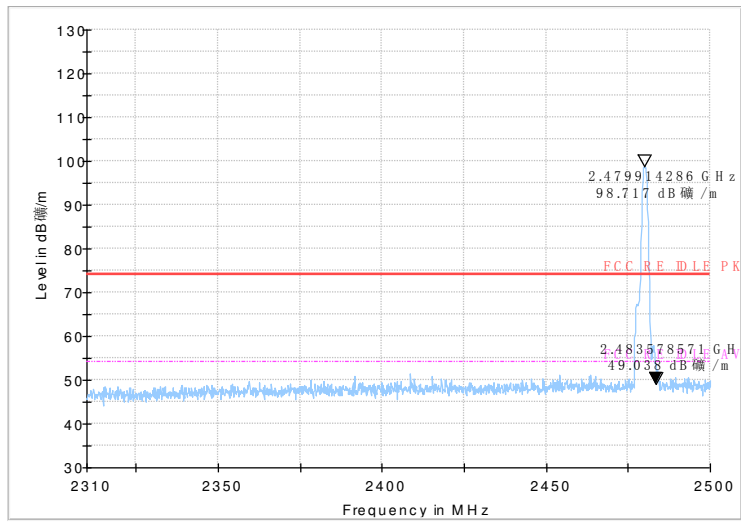
Fig.44 Radiated emission (Power): GFSK, high channel
