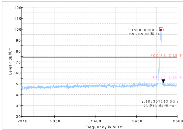
Fig.50 Radiated emission (Power): \pi/4 DQPSK, high channel
