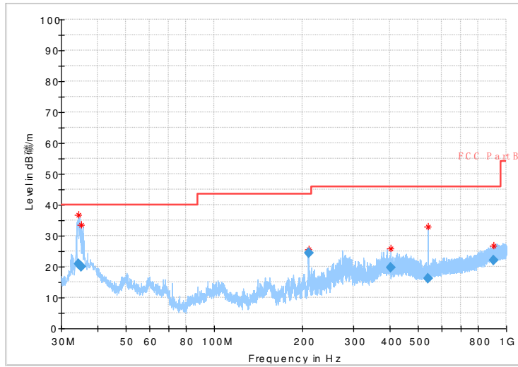
Fig.46 Radiated emission: \pi/4 DQPSK, Ch78, 30MHz~1GHz
