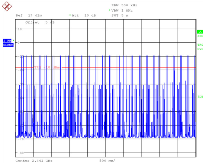
Fig.64 Time of occupancy (Dwell Time): Ch39, Packet 2-DH1
