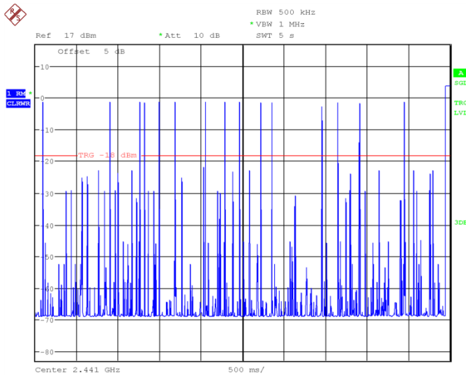
Fig.68 Time of occupancy (Dwell Time): Ch39, Packet 2-DH5
