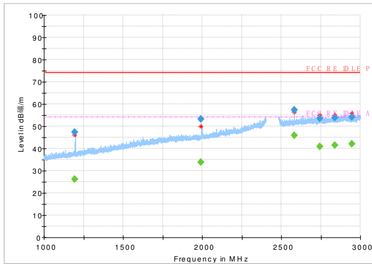
Fig.47 Radiated emission: \pi/4 DQPSK, Ch78, 1GHz~3GHz
