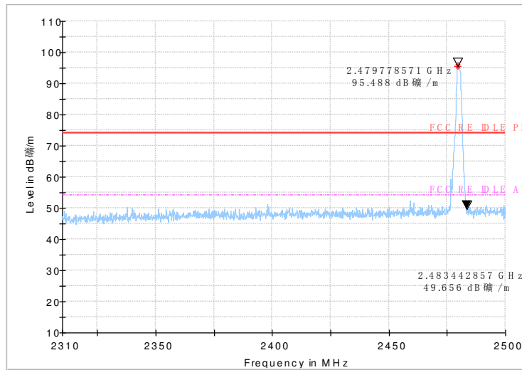
Fig.56 Radiated emission (Power): 8DPSK, high channel
