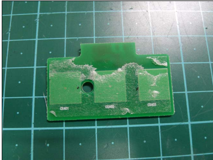
Bottom view of TOUCH PCB
