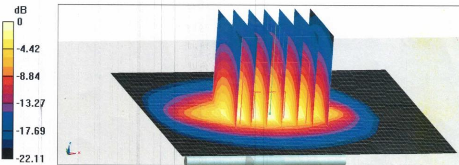
0 dB = 21.9 W/kg = 13.40 dBW/kg
